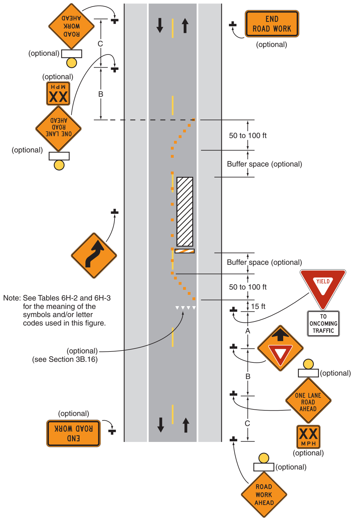
Typical Application 11
