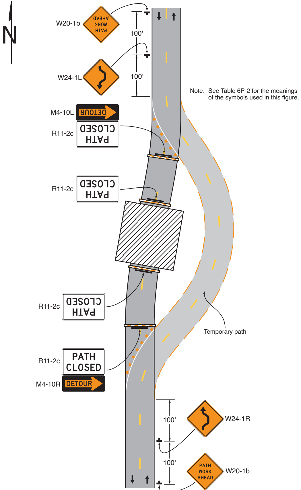
Typical Application 49
