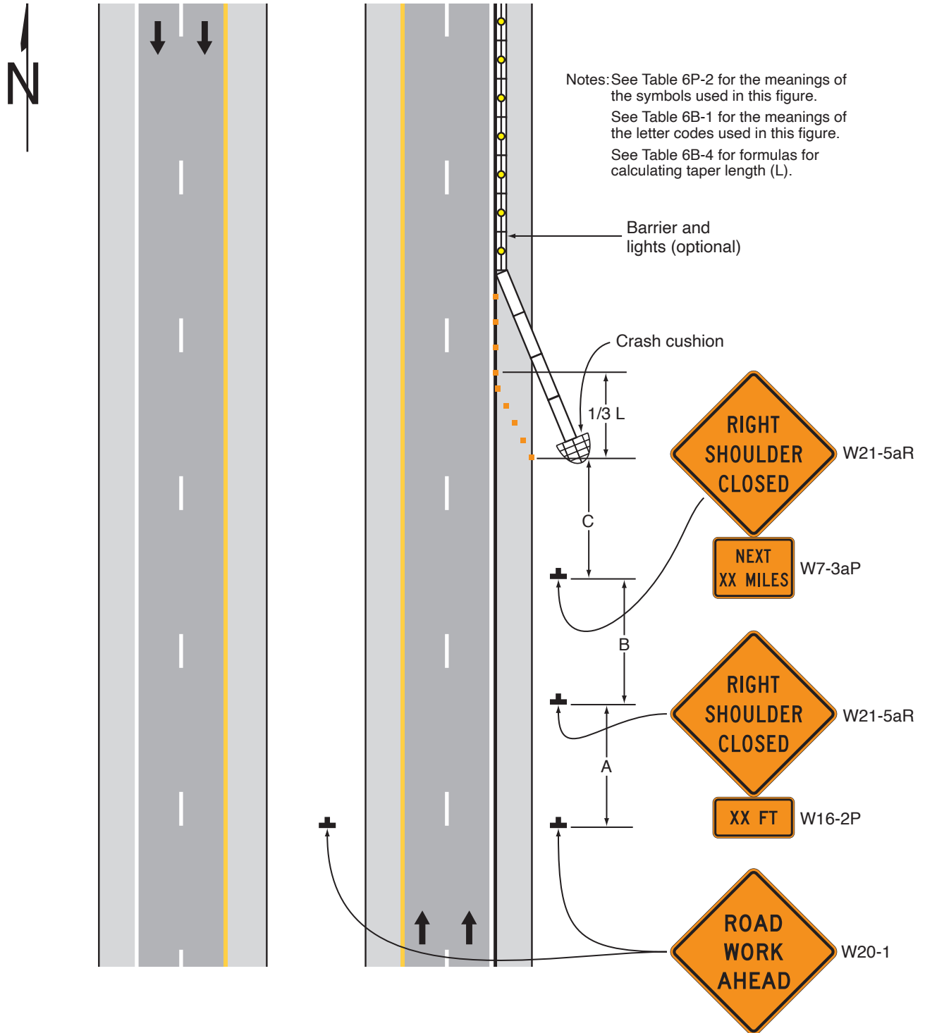
Typical Application 5
