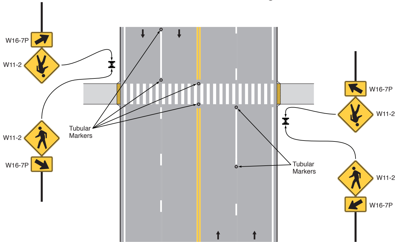
Figure 2 – Tubular Markers Supplementing Centerline and Lane Line Markings
