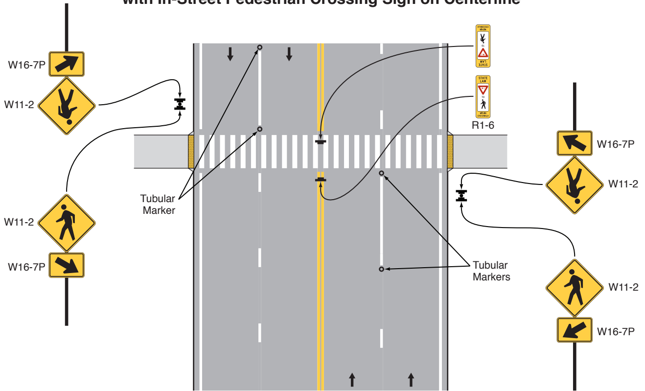
Figure 3 – Tubular Markers Supplementing Lane Lines with In-Street Pedestrian Crossing Sign on Centerline
