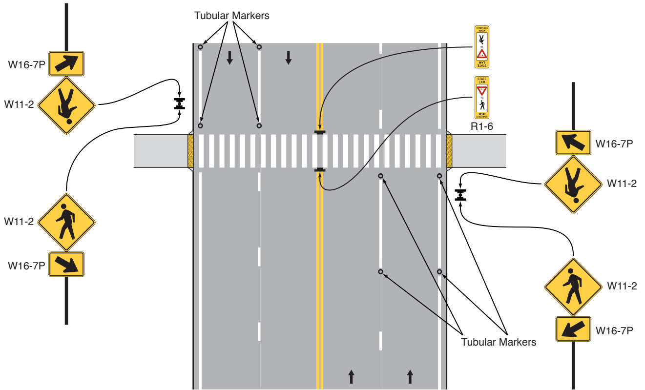
Figure 4 – Tubular Markers Supplementing Edge and Lane Lines; In-Street Pedestrian Sign Crossing on Centerline
