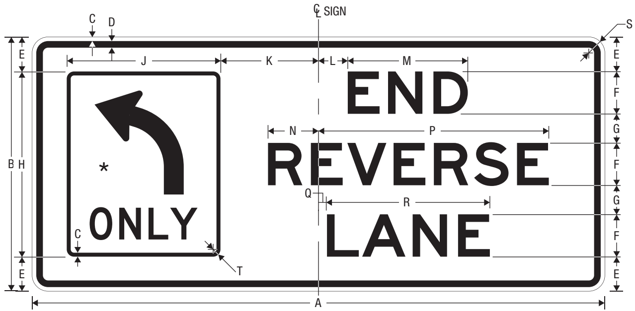
R3-9i END REVERSE LANE
