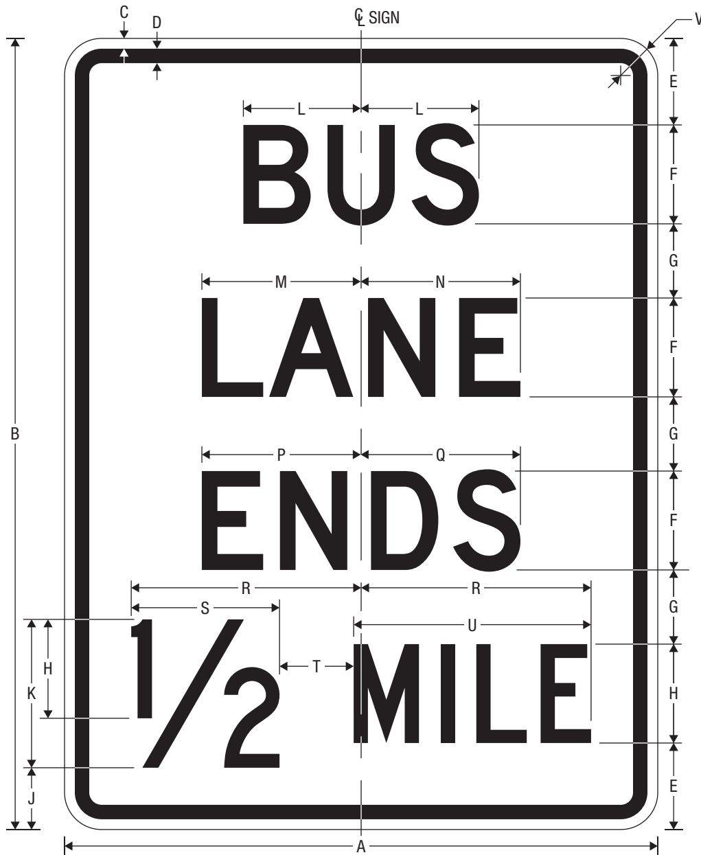
R3-12h PREFERENTIAL LANE ENDS (POST-MOUNTED)
