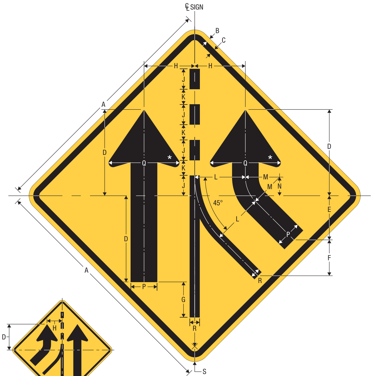
W4-3R ADDED LANE
