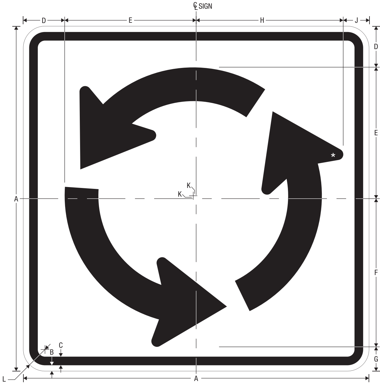
R6-5P ROUNDABOUT CIRCULATION (PLAQUE)
