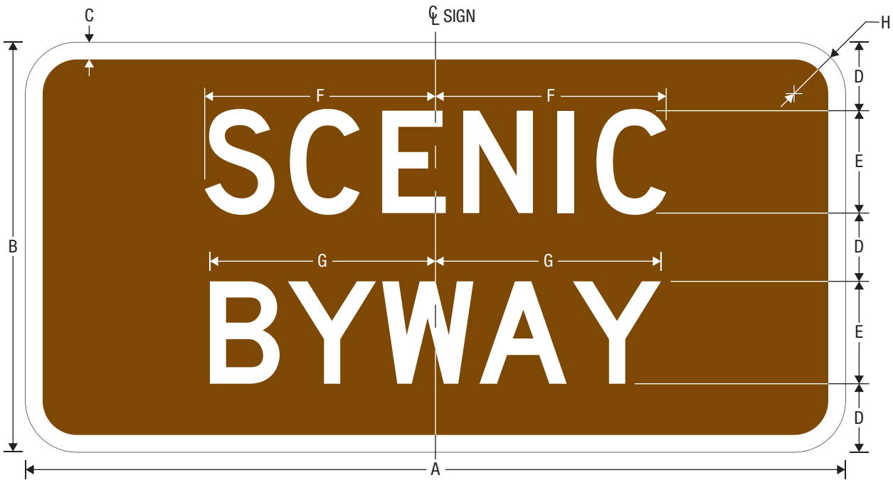
M10-3bP SCENIC BYWAY (PLAQUE)
