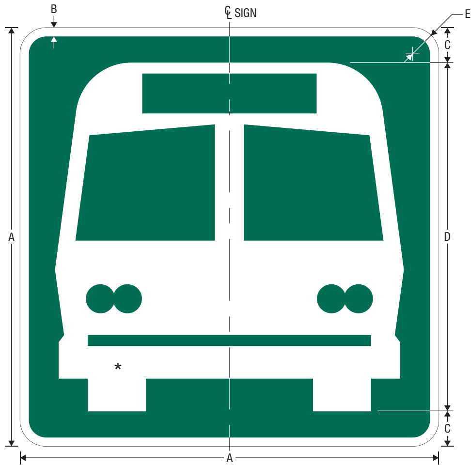
I3-6 BUS STATION
