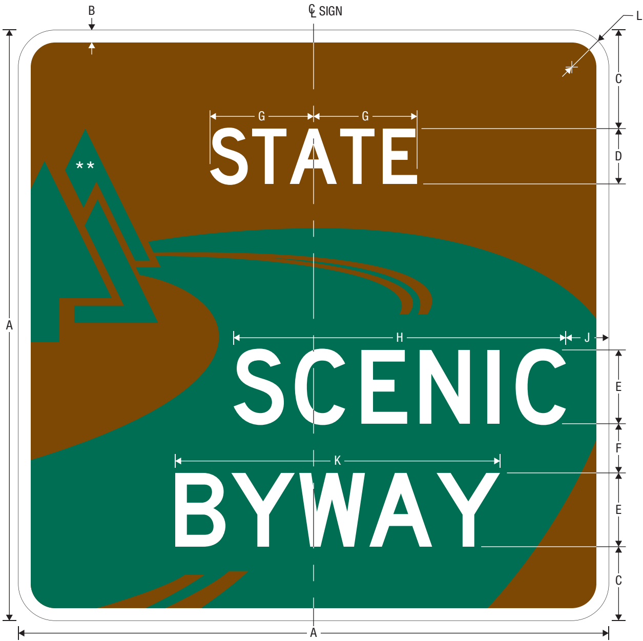
M10-3 STATE SCENIC BYWAY SYSTEM
