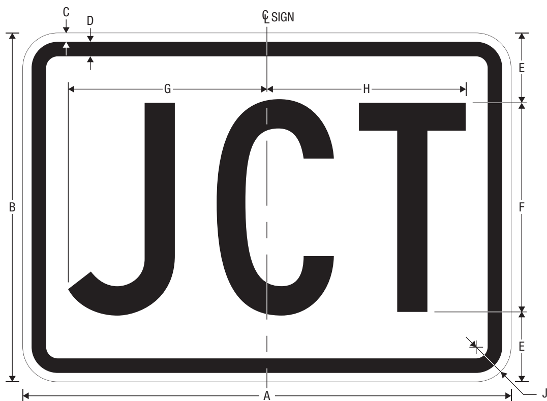
M2-1P JUNCTION (PLAQUE)
