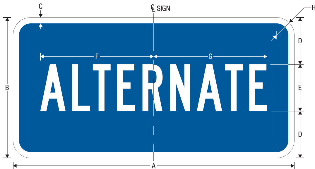
M4-1P ALTERNATE (PLAQUE)
