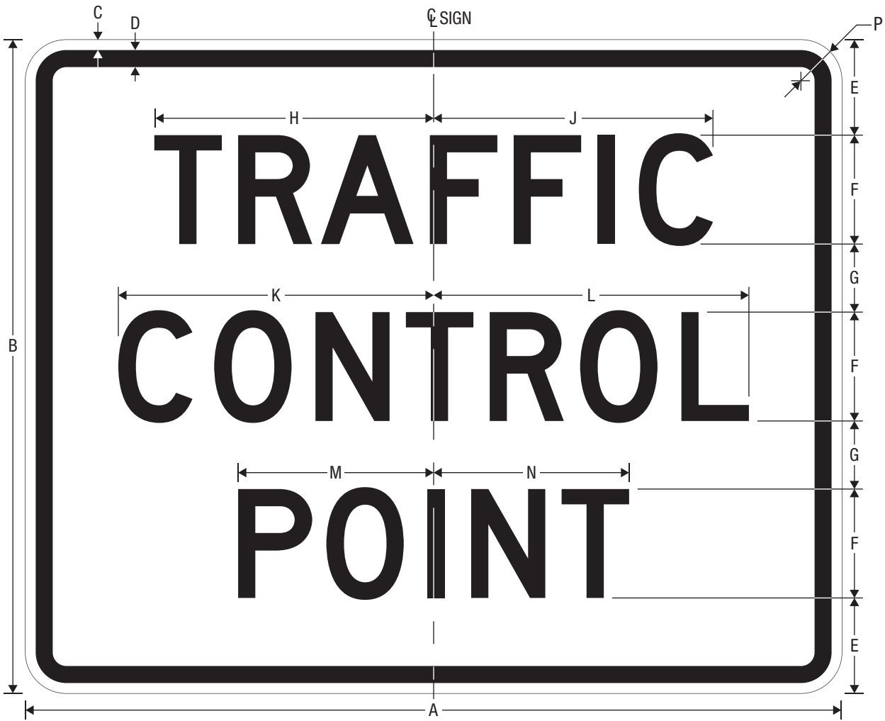
EM2-2 TRAFFIC CONTROL POINT
