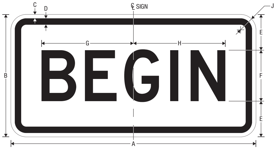
M4-14P BEGIN (PLAQUE)
