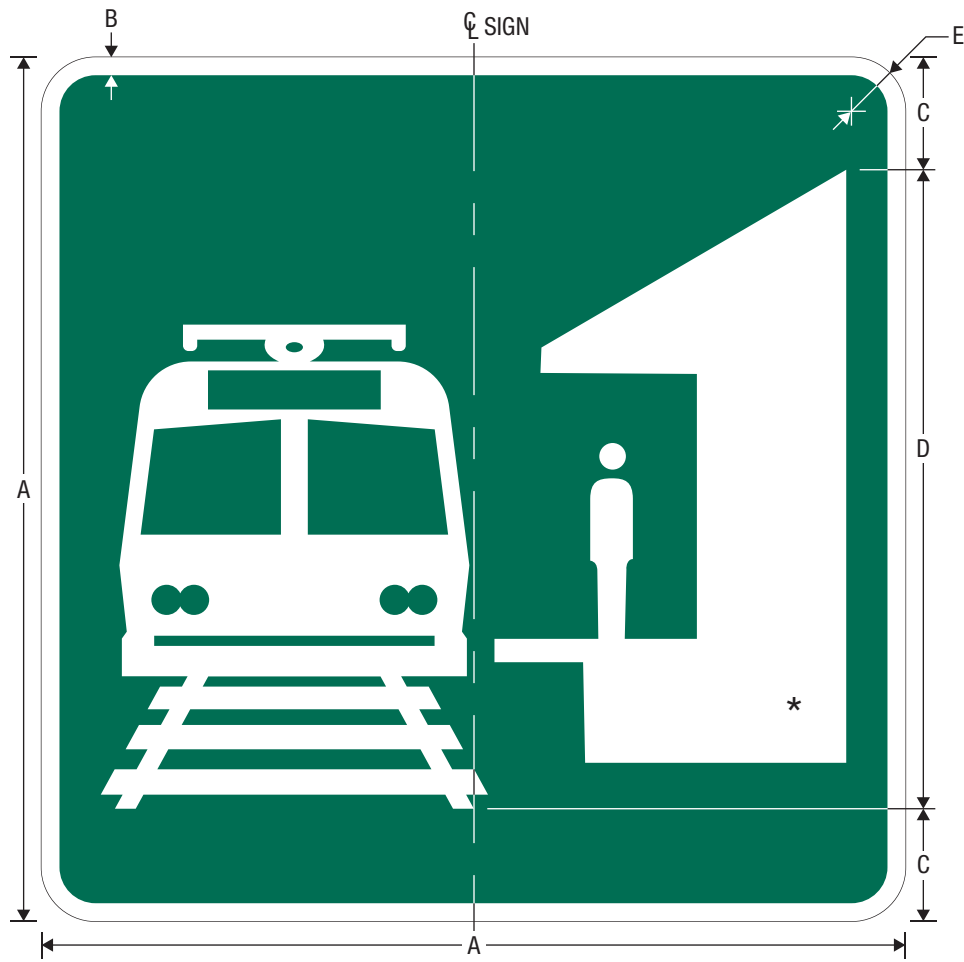
I3-8 LIGHT RAIL TRANSIT STATION
