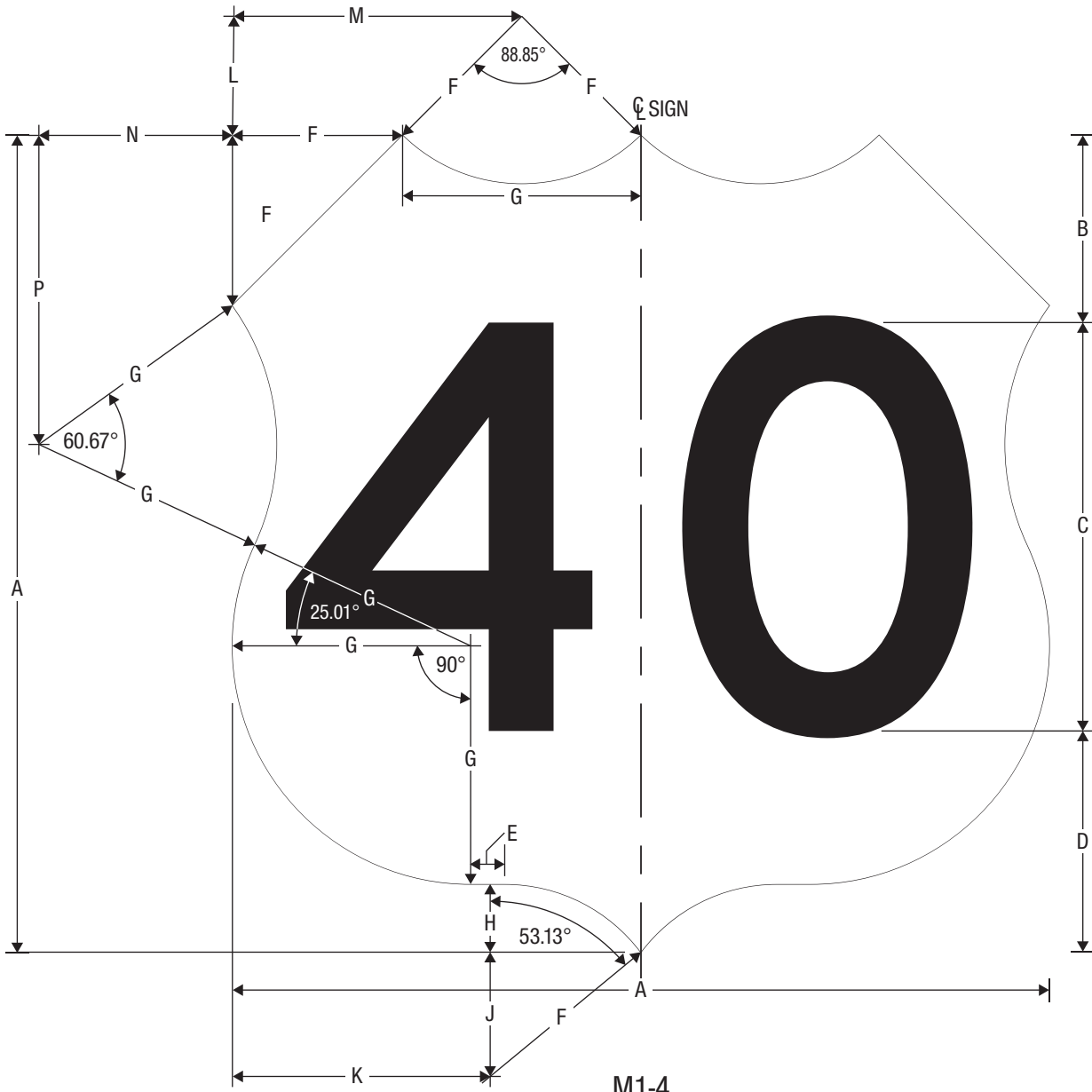
M1-4 U.S. ROUTE - GUIDE SIGN USE (1, 2 DIGITS)
