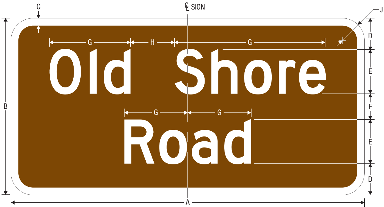
M10-2aP BYWAY IDENTIFICATION (PLAQUE)
