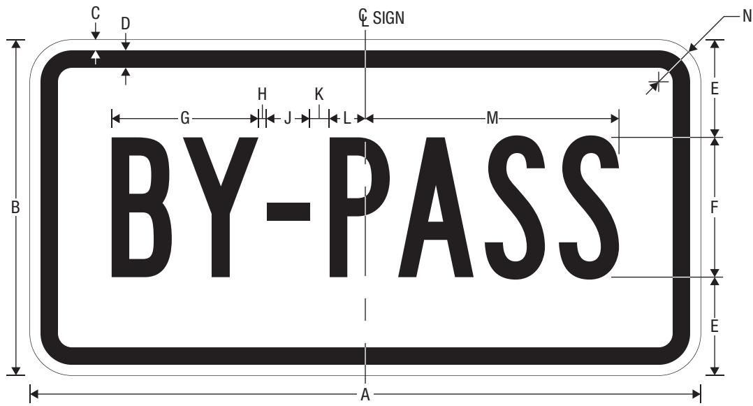
M4-2P BY-PASS (PLAQUE)
