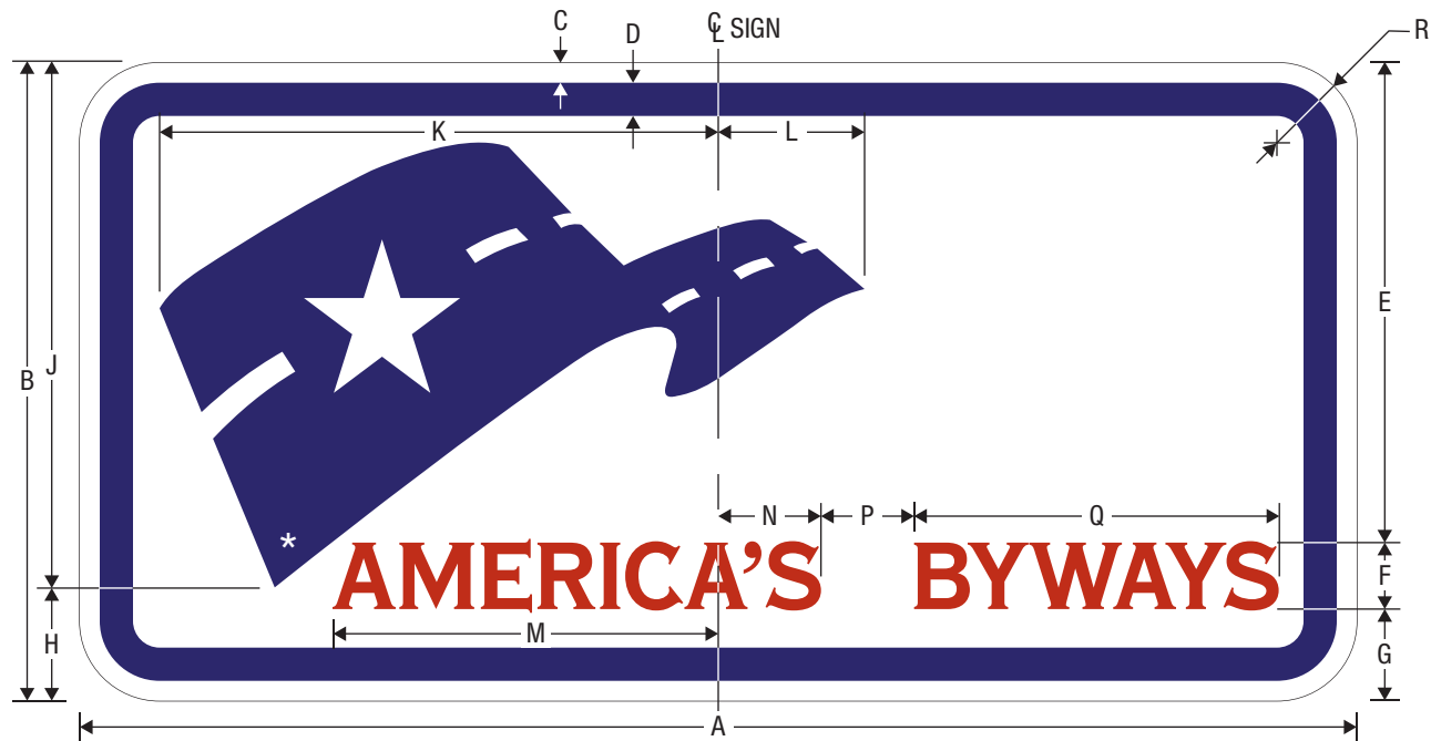
M10-1aP NATIONAL SCENIC BYWAY (PLAQUE)
