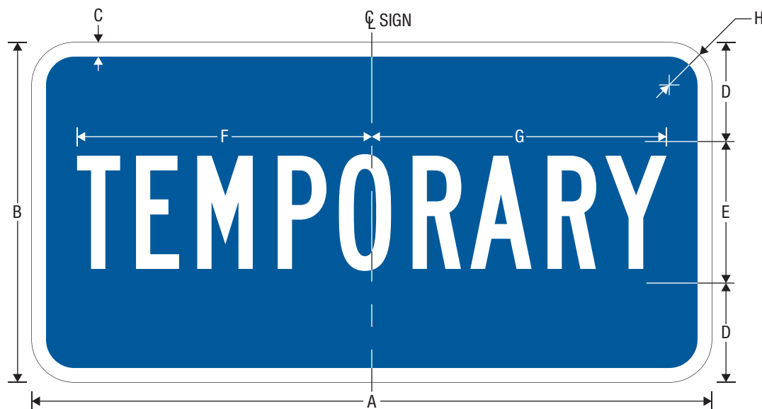
M4-7P TEMPORARY (PLAQUE)
