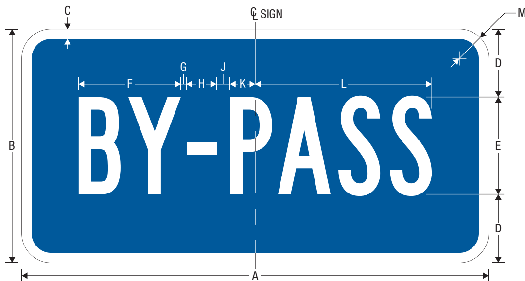
M4-2P BY-PASS (PLAQUE)
