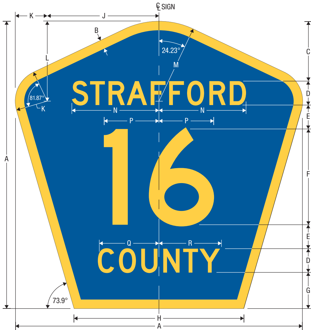
M1-6 COUNTY ROUTE
