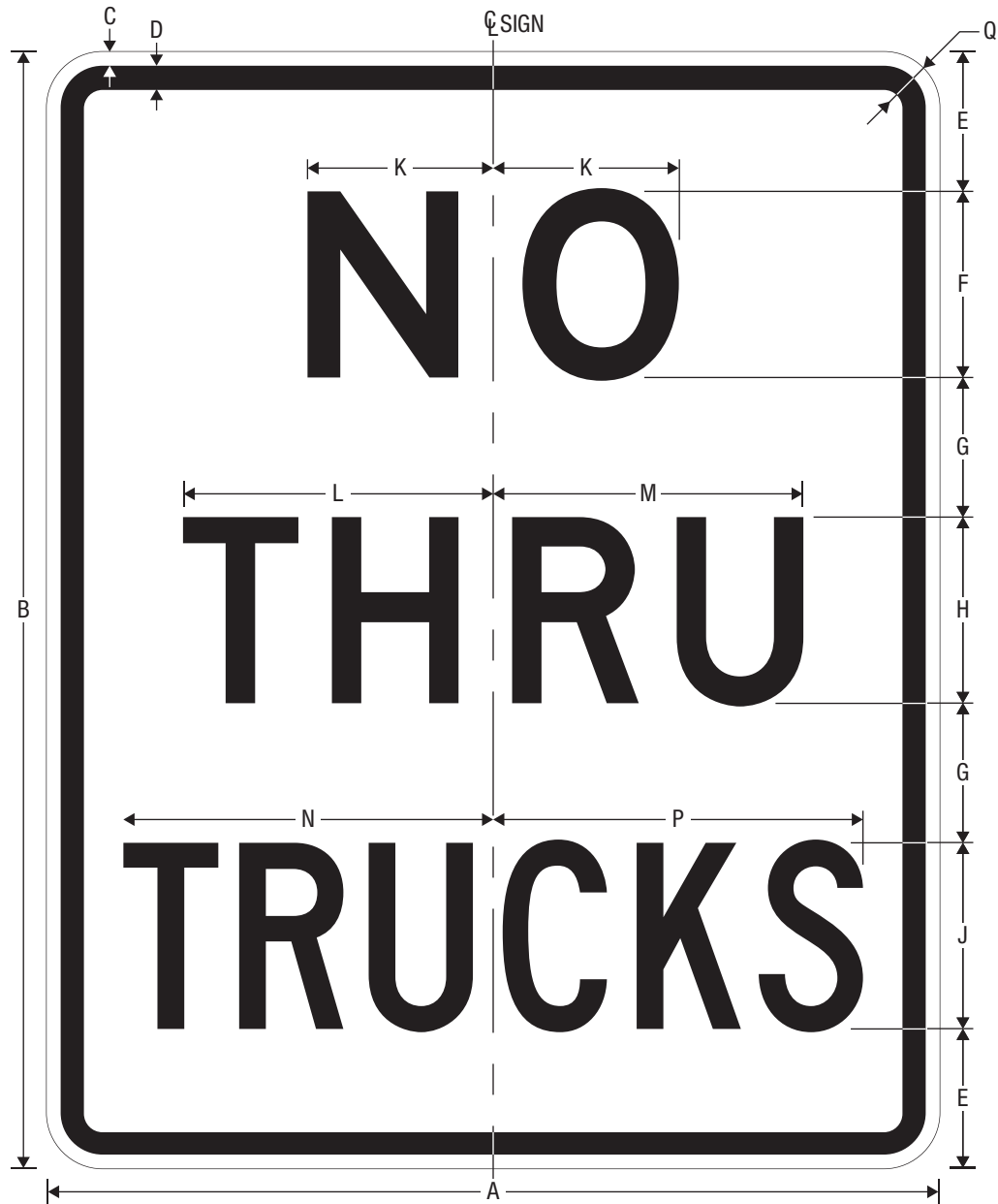
R5-2b NO THRU TRUCKS
