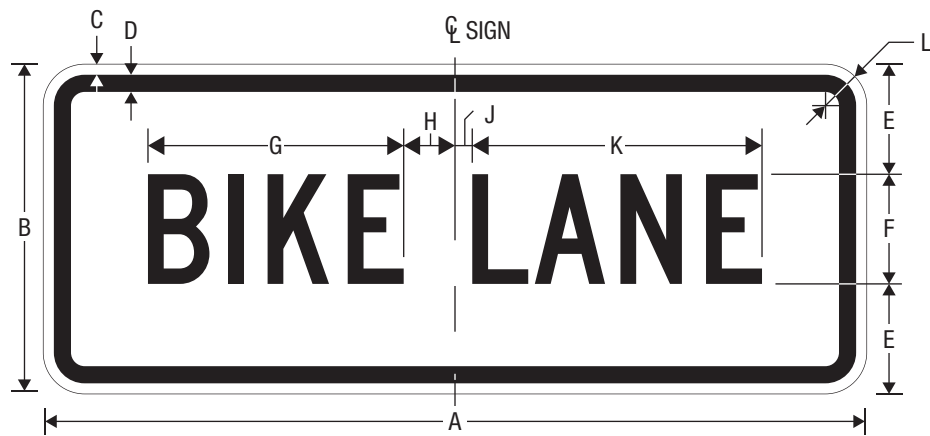
R3-5hP BIKE LANE (PLAQUE)
