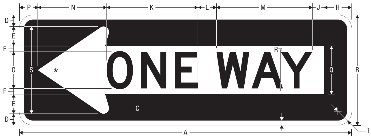
R6-1L ONE WAY
