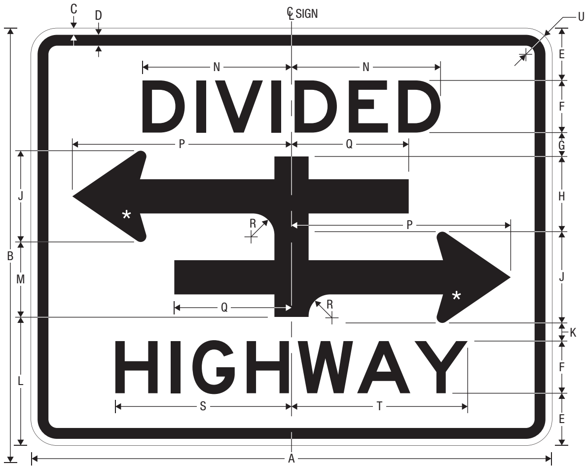
R6-3 DIVIDED HIGHWAY CROSSING
