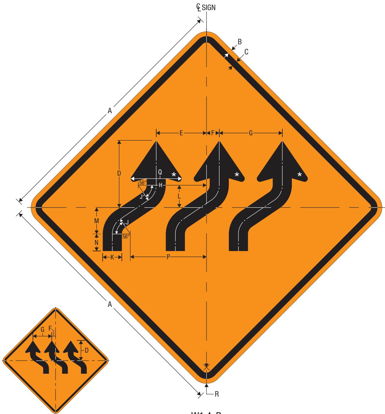
W1-4cR REVERSE CURVE (3 LANES)
