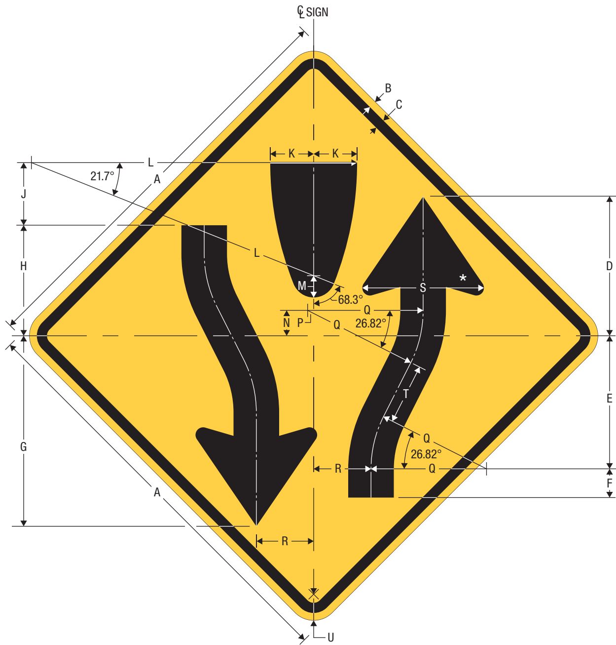
W6-1 DIVIDED HIGHWAY
