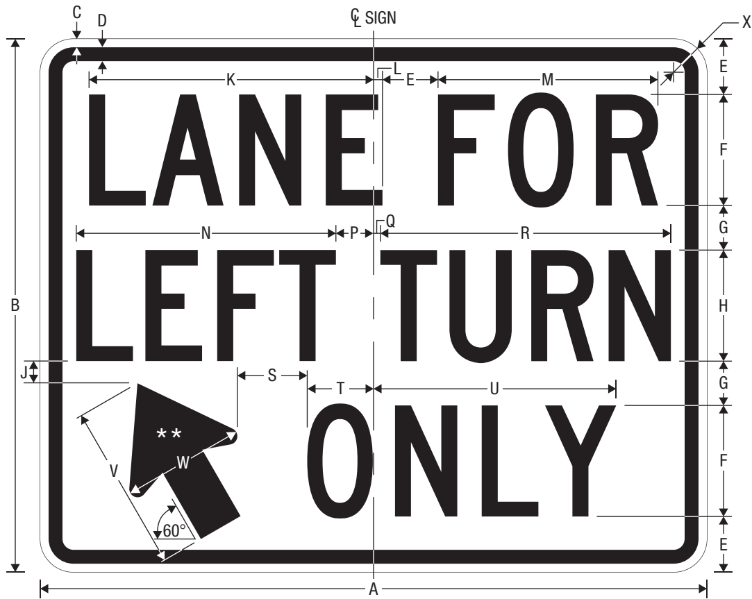
R3-19 LANE FOR LEFT TURN ONLY
