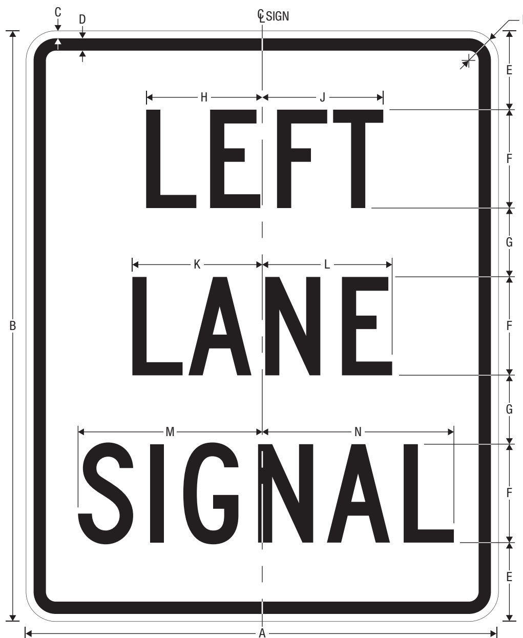
R10-10bL LEFT LANE SIGNAL
