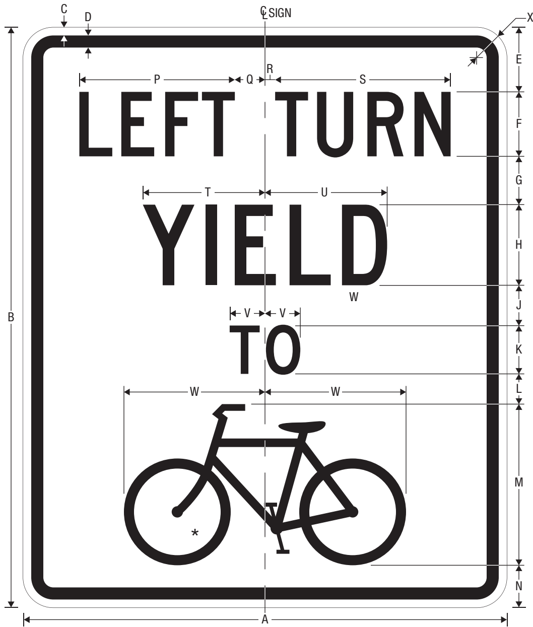
R10-12b LEFT TURN YIELD TO BICYCLE
