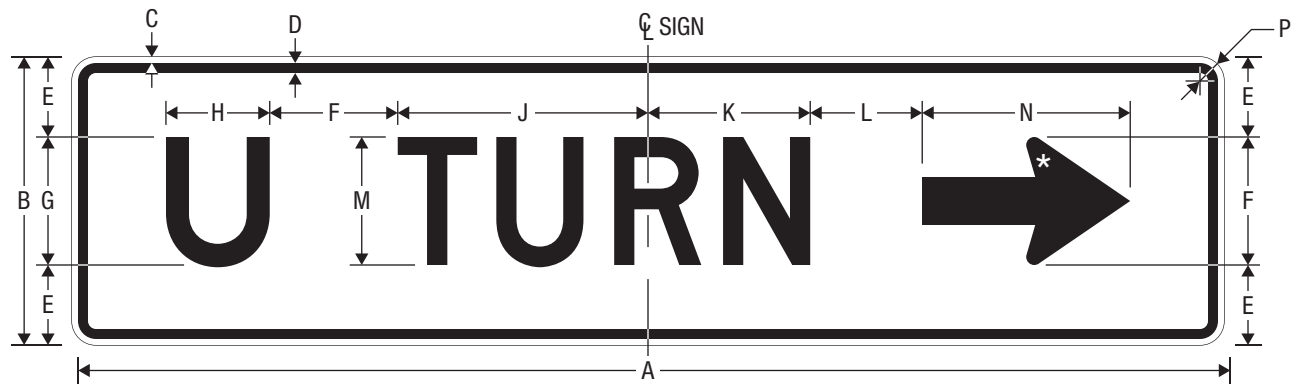
R3-25b U TURN DIRECTIONAL
