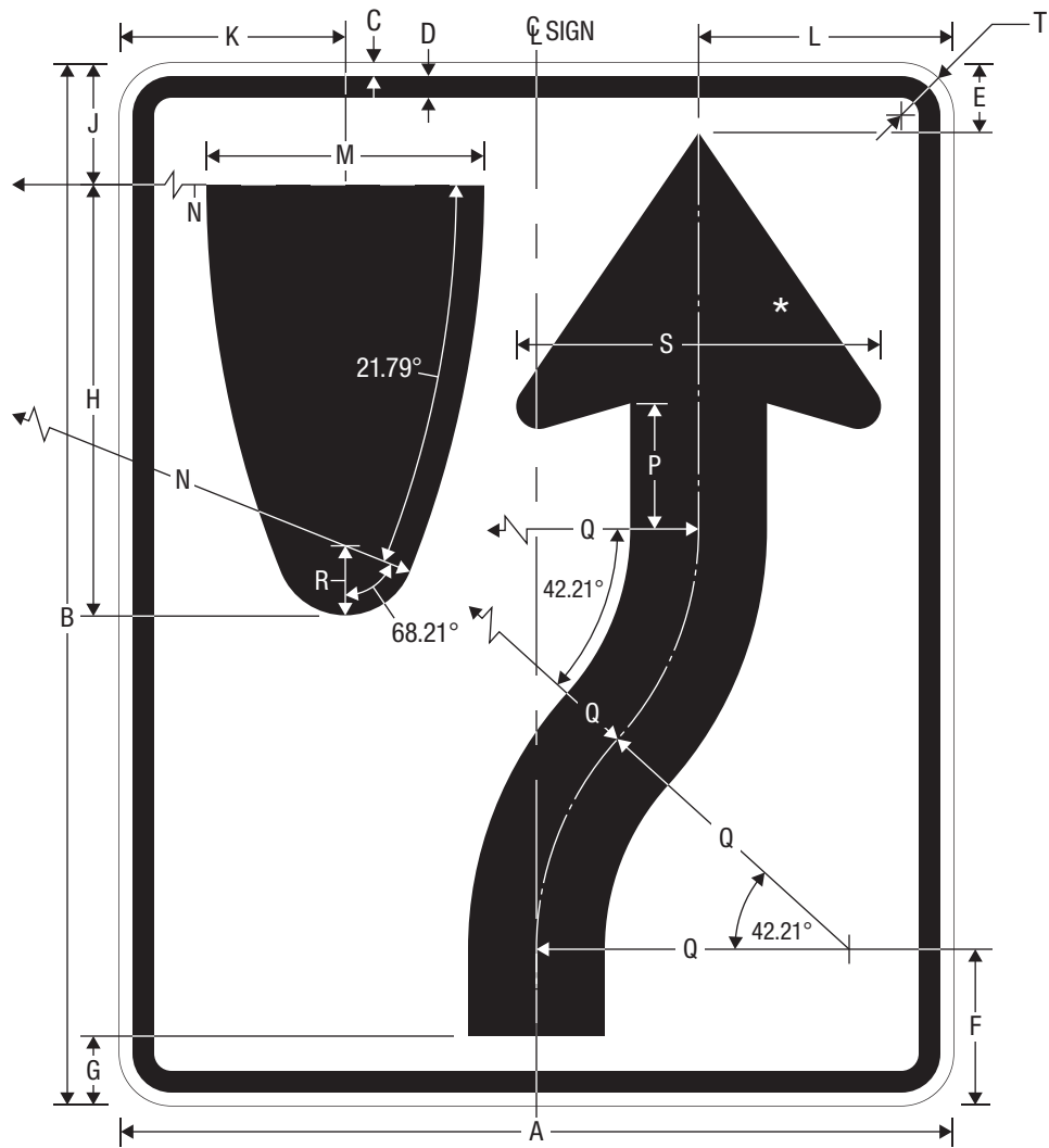
R4-7 KEEP RIGHT
