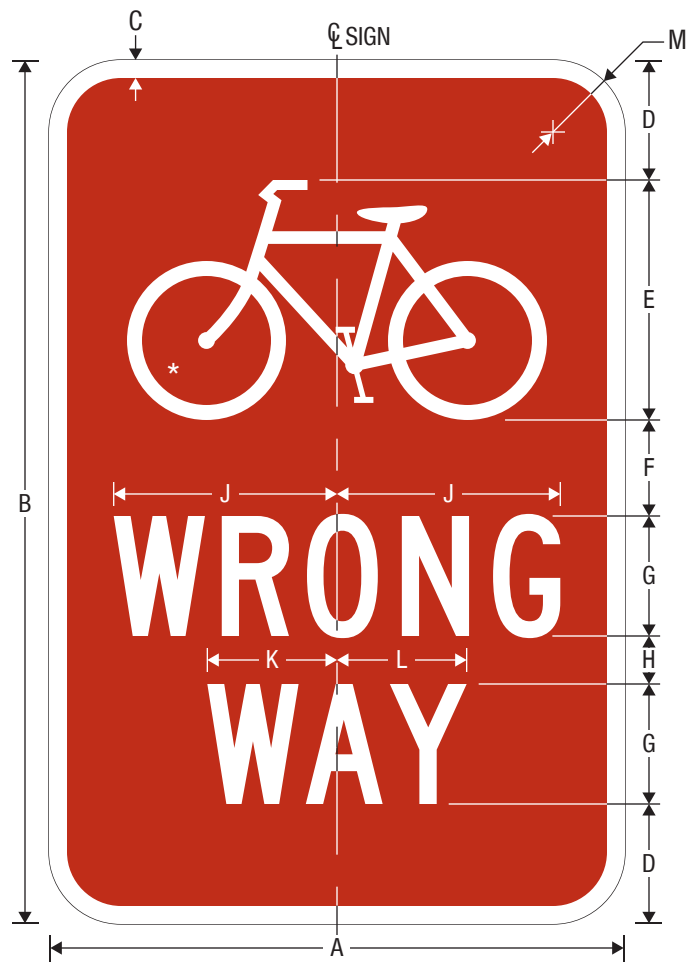
R5-1b BICYCLE WRONG WAY
