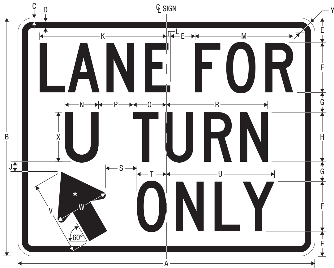
R3-19a LANE FOR U TURN ONLY
