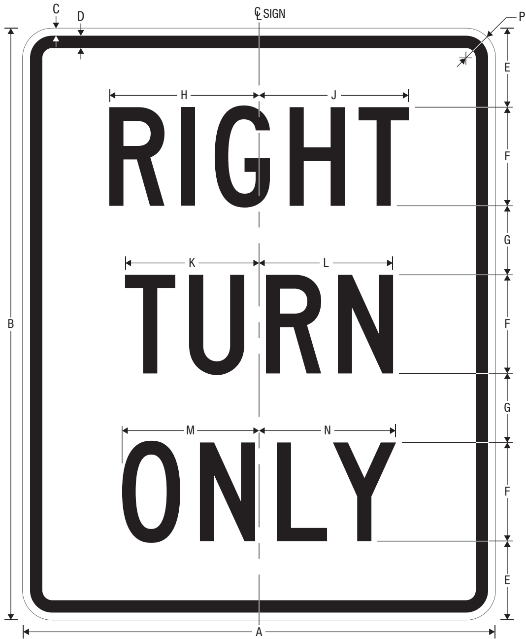
R4-21R RIGHT TURN ONLY
