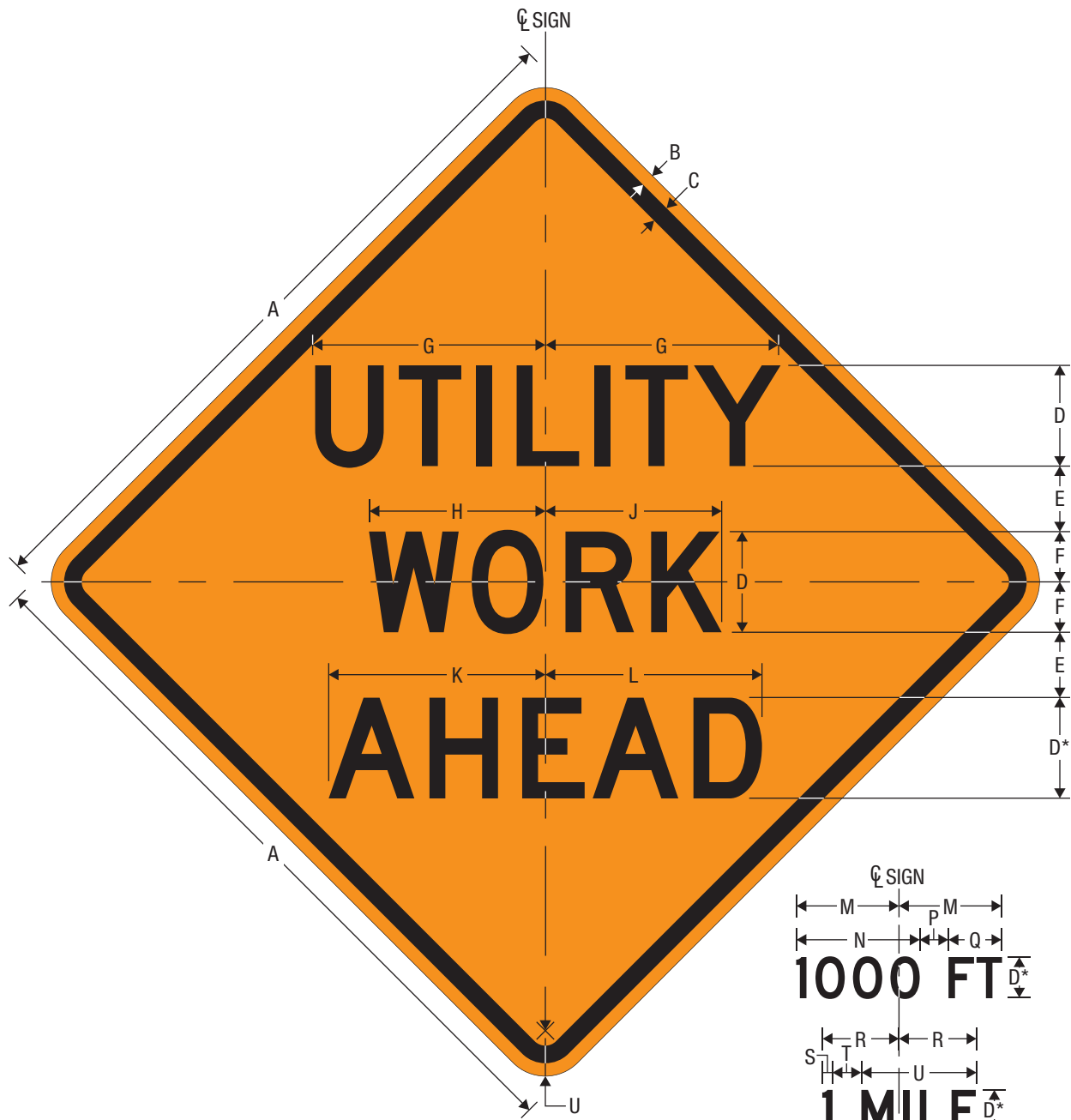
W21-7 UTILITY WORK (WITH DISTANCE)
