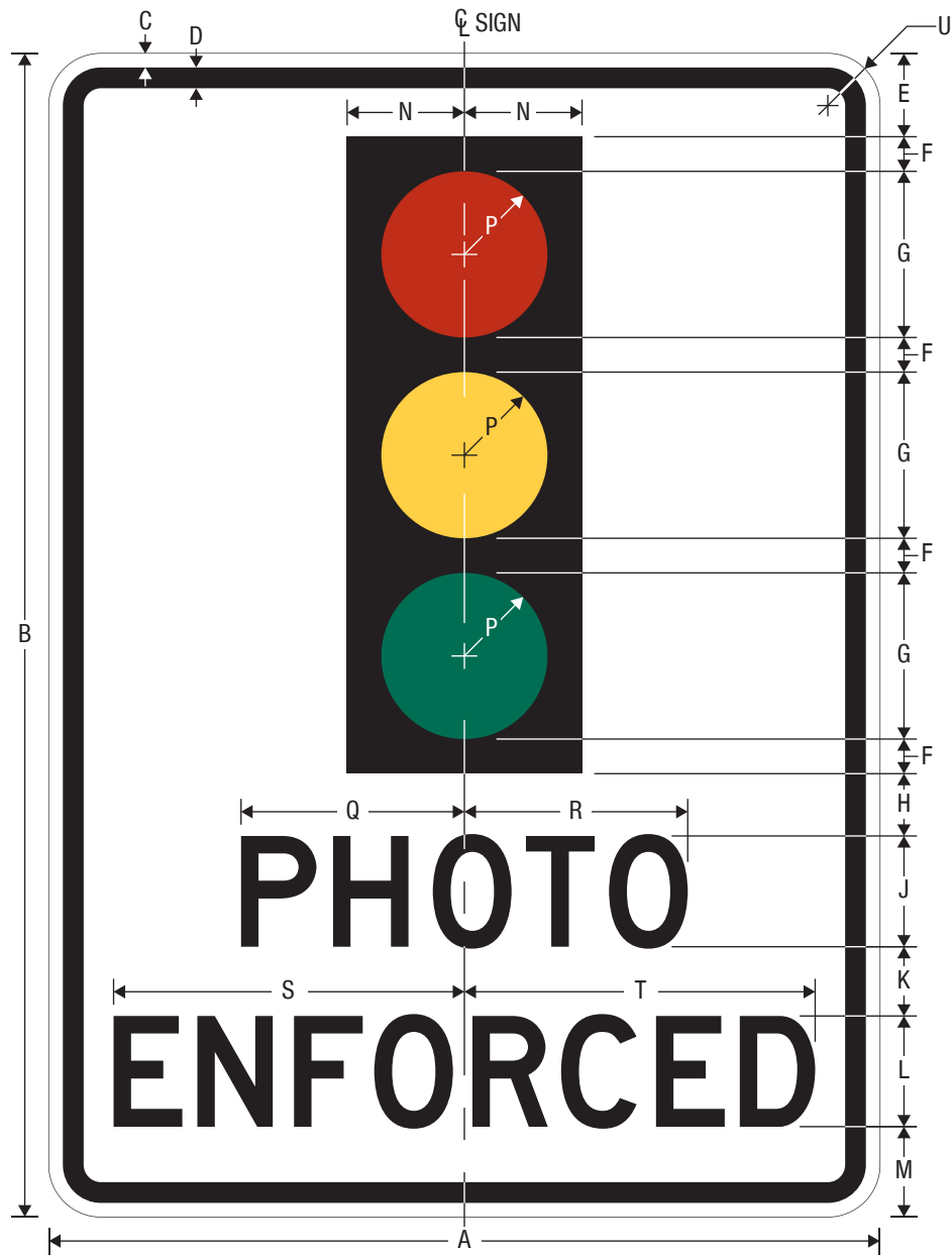
R10-18a TRAFFIC SIGNAL PHOTO ENFORCED
