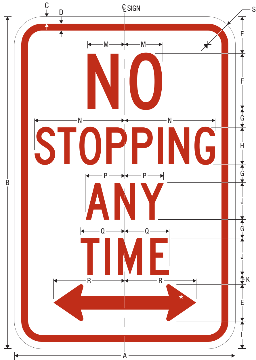
R7-4a NO STOPPING ANY TIME
