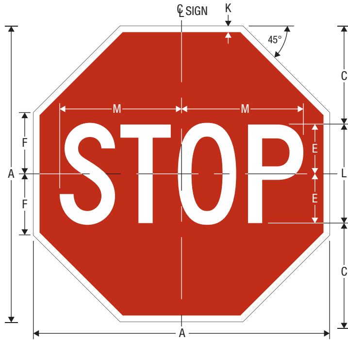
R1-1 STOP (ON STOP/SLOW PADDLE)
