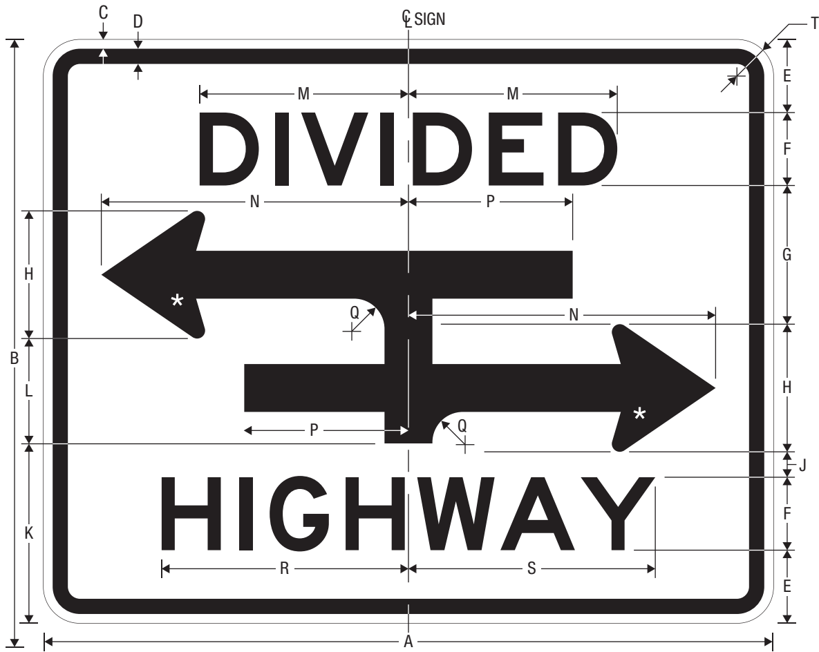
R6-3a DIVIDED HIGHWAY CROSSING
