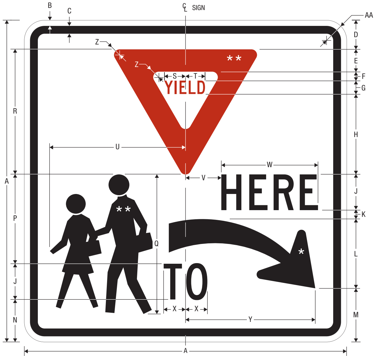
R1-5aR YIELD HERE TO SCHOOL CROSSING
