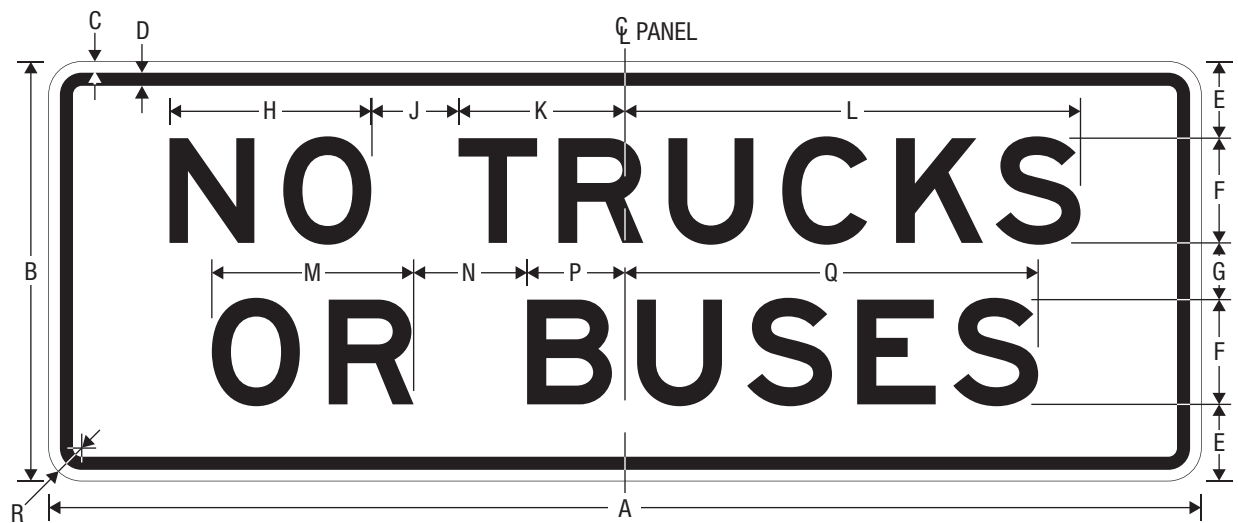
R3-51bP NO TRUCKS OR BUSES (PLAQUE)
