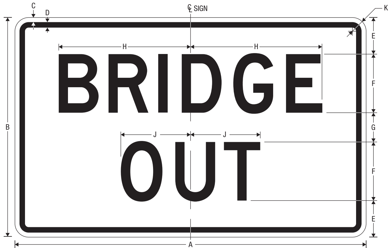
R11-2b BRIDGE OUT
