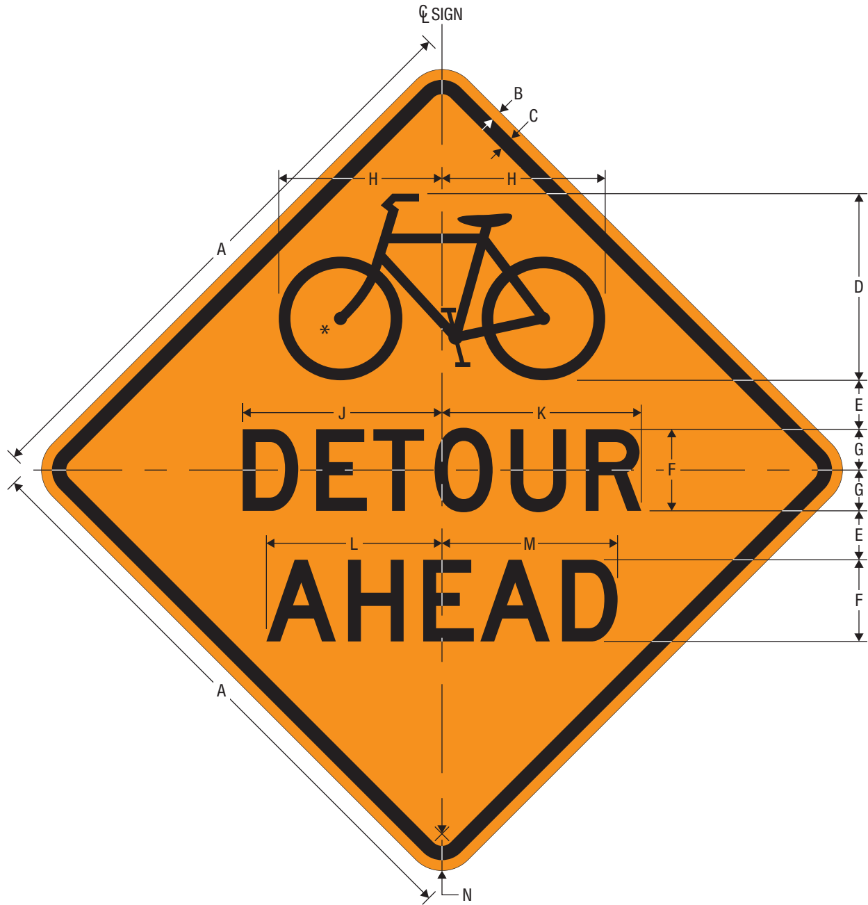
W20-2a BIKE DETOUR (WITH DISTANCE)
