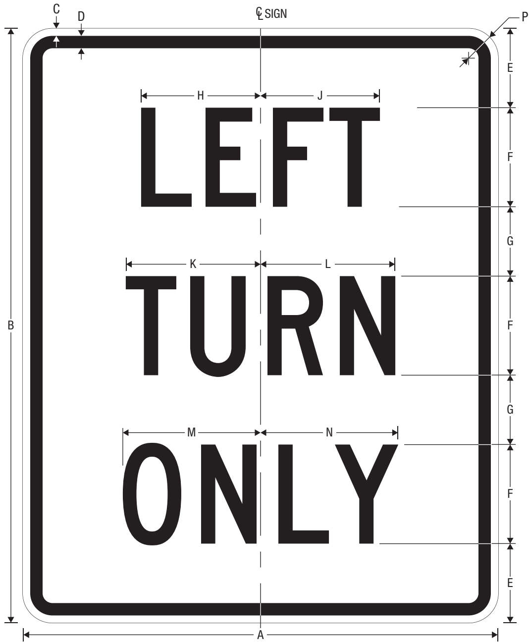
R4-21L LEFT TURN ONLY
