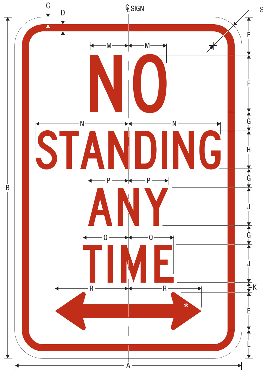
R7-4 NO STANDING ANY TIME
