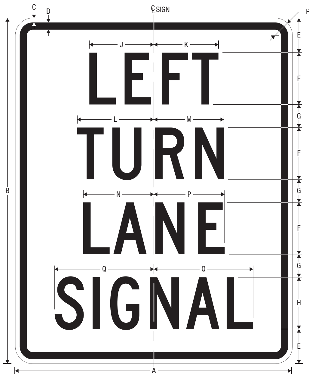
R10-10cL LEFT TURN LANE SIGNAL
