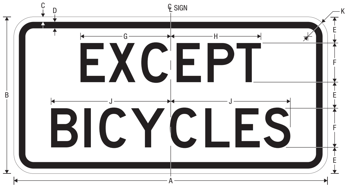
R3-7bP EXCEPT BICYCLES (PLAQUE)
