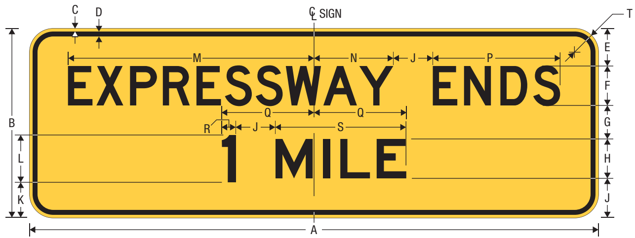
W19-2 EXPRESSWAY ENDS XX MILES
