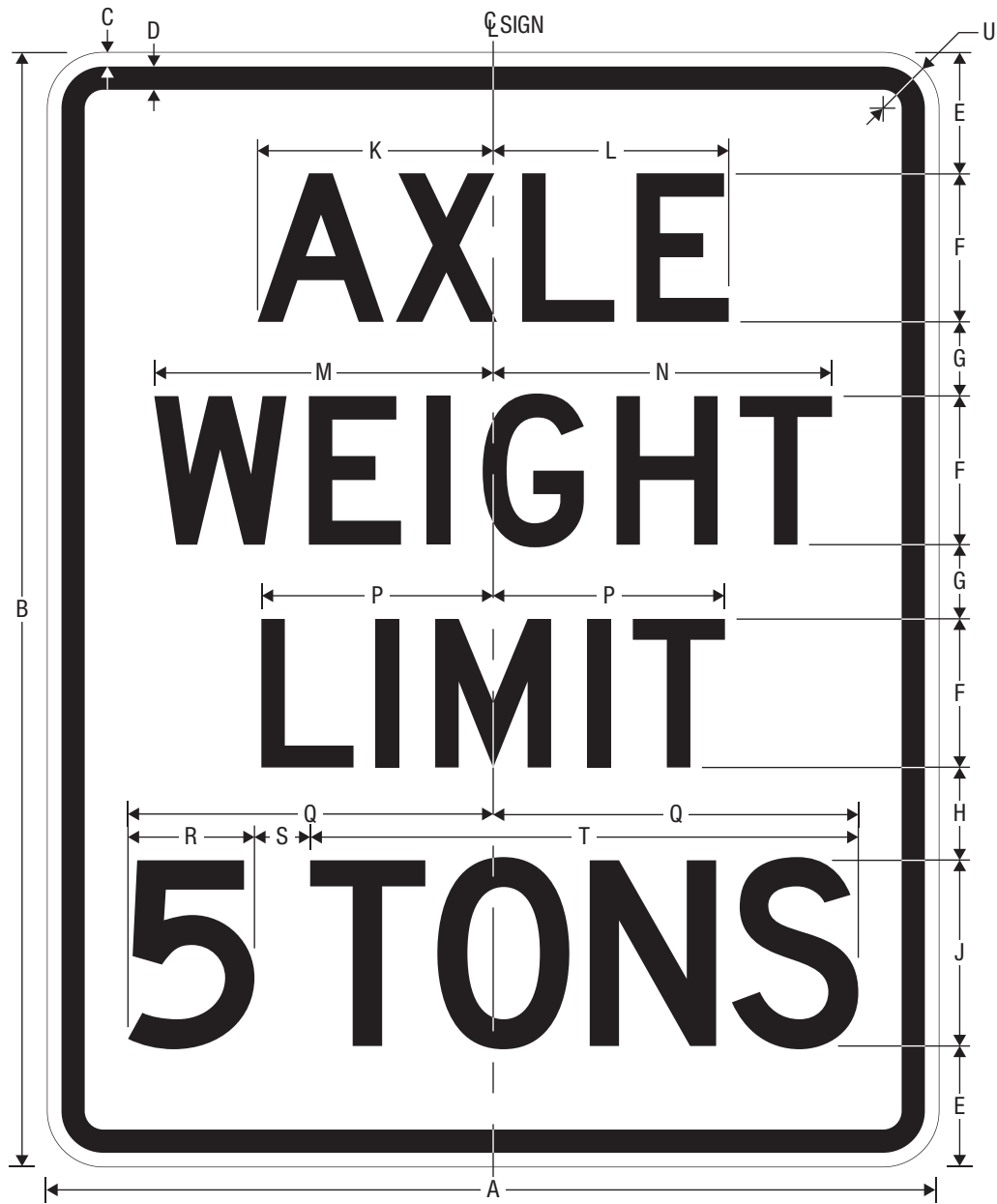
R12-2 WEIGHT LIMIT
