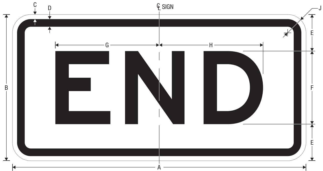
R3-9dP END (PLAQUE)
