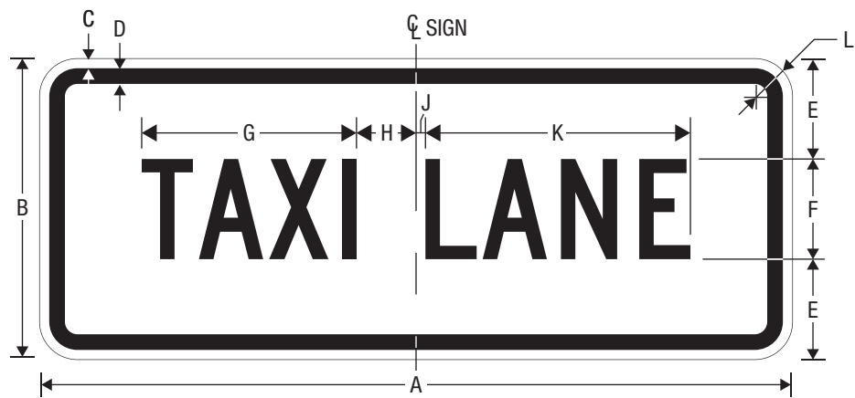
R3-5dP TAXI LANE (PLAQUE)
