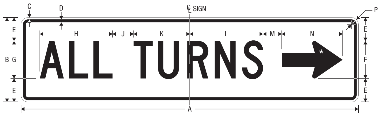
R3-25 ALL TURNS DIRECTIONAL
