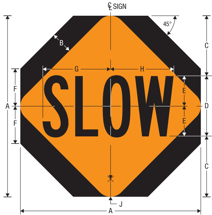
W20-8 SLOW (ON STOP/SLOW PADDLE)
