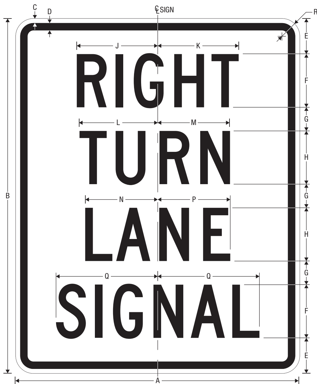
R10-10cR RIGHT TURN LANE SIGNAL
