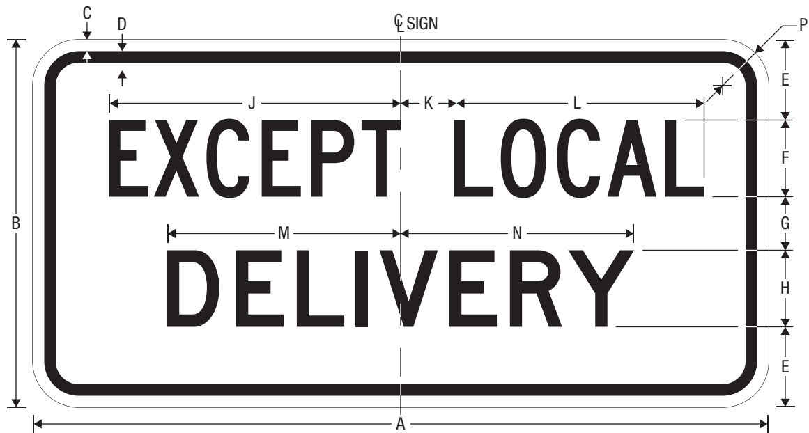
R5-2aP EXCEPT LOCAL DELIVERY (PLAQUE)
