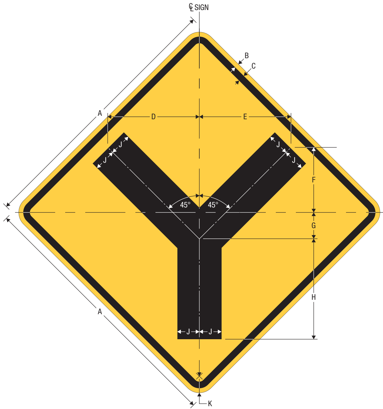
W2-5 INTERSECTION WARNING - Y-INTERSECTION
