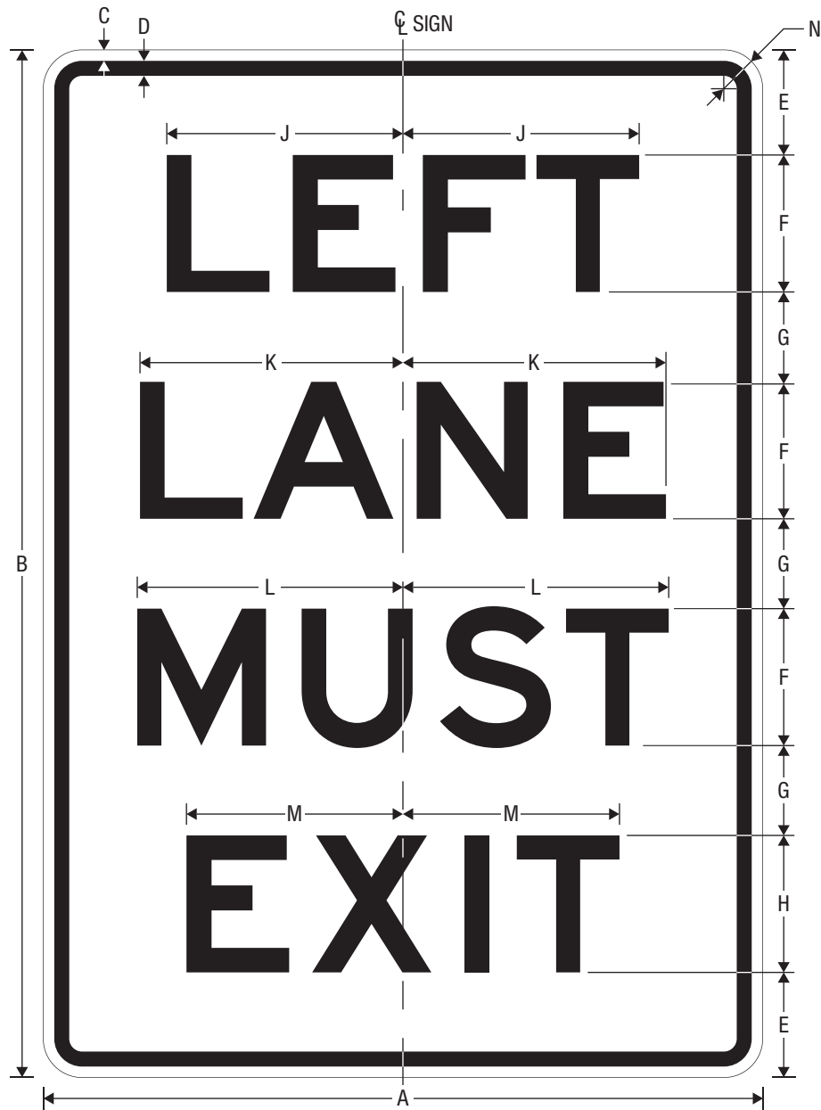
R3-33aL LEFT LANE MUST EXIT
