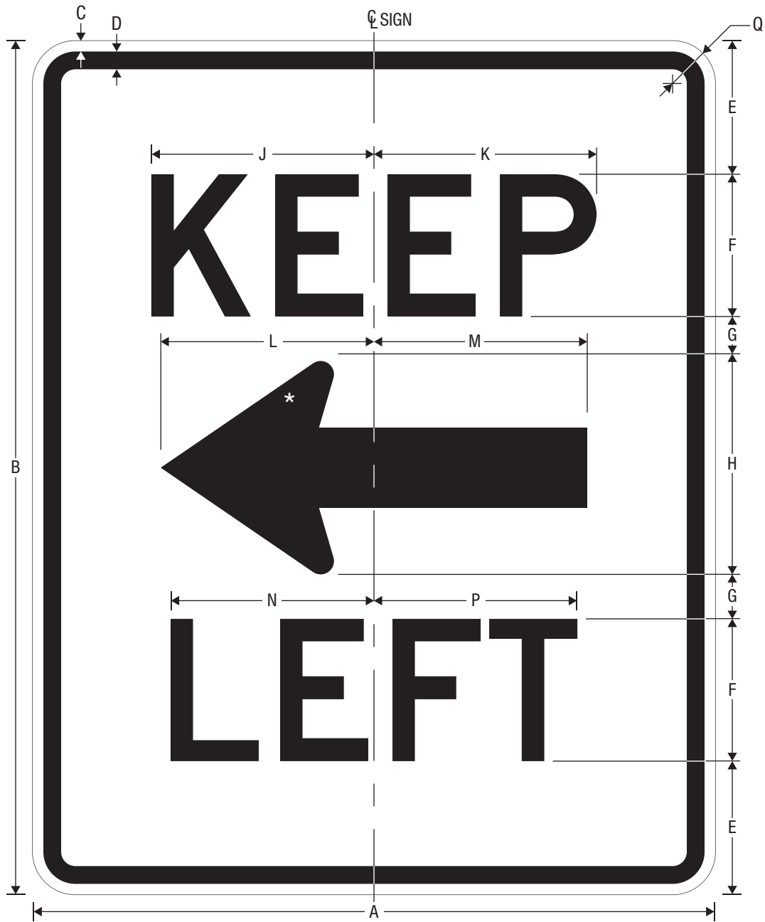
R4-8a KEEP LEFT
