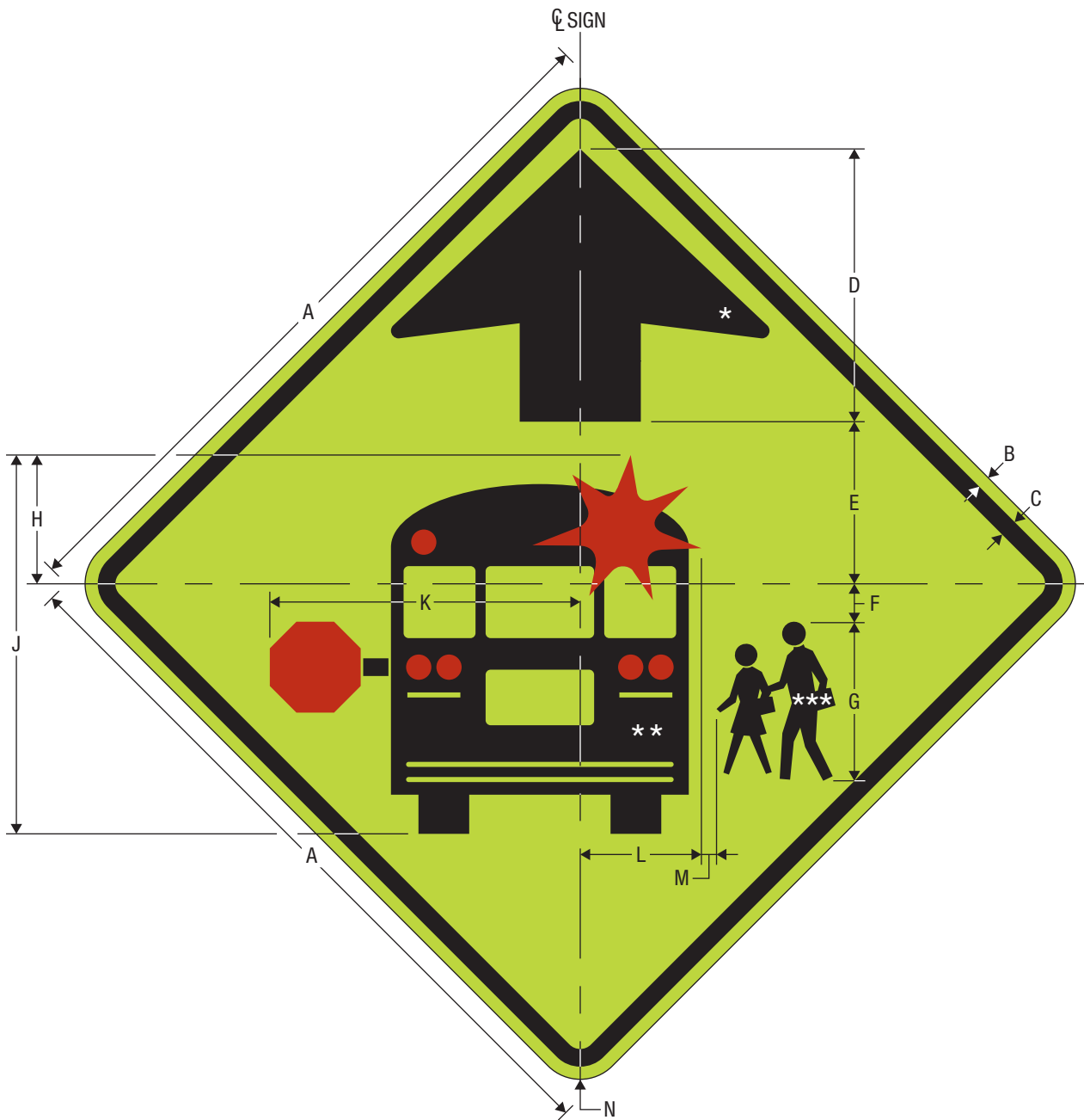
S3-1 SCHOOL BUS STOP AHEAD
