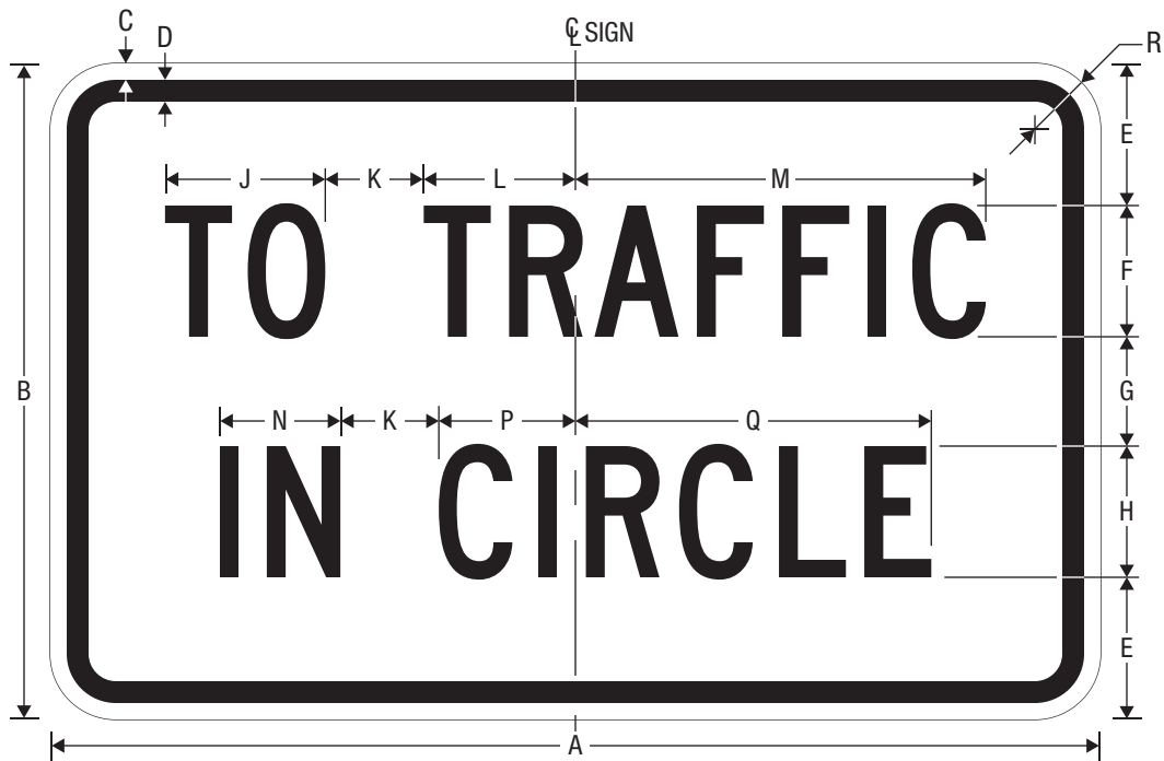
R1-2bP TO TRAFFIC IN CIRCLE (PLAQUE)
