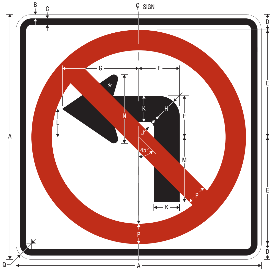
R3-2 MOVEMENT PROHIBITION - NO LEFT TURN
