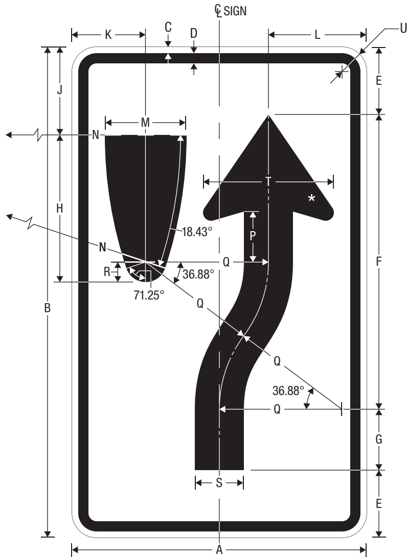
R4-7c NARROW KEEP RIGHT
