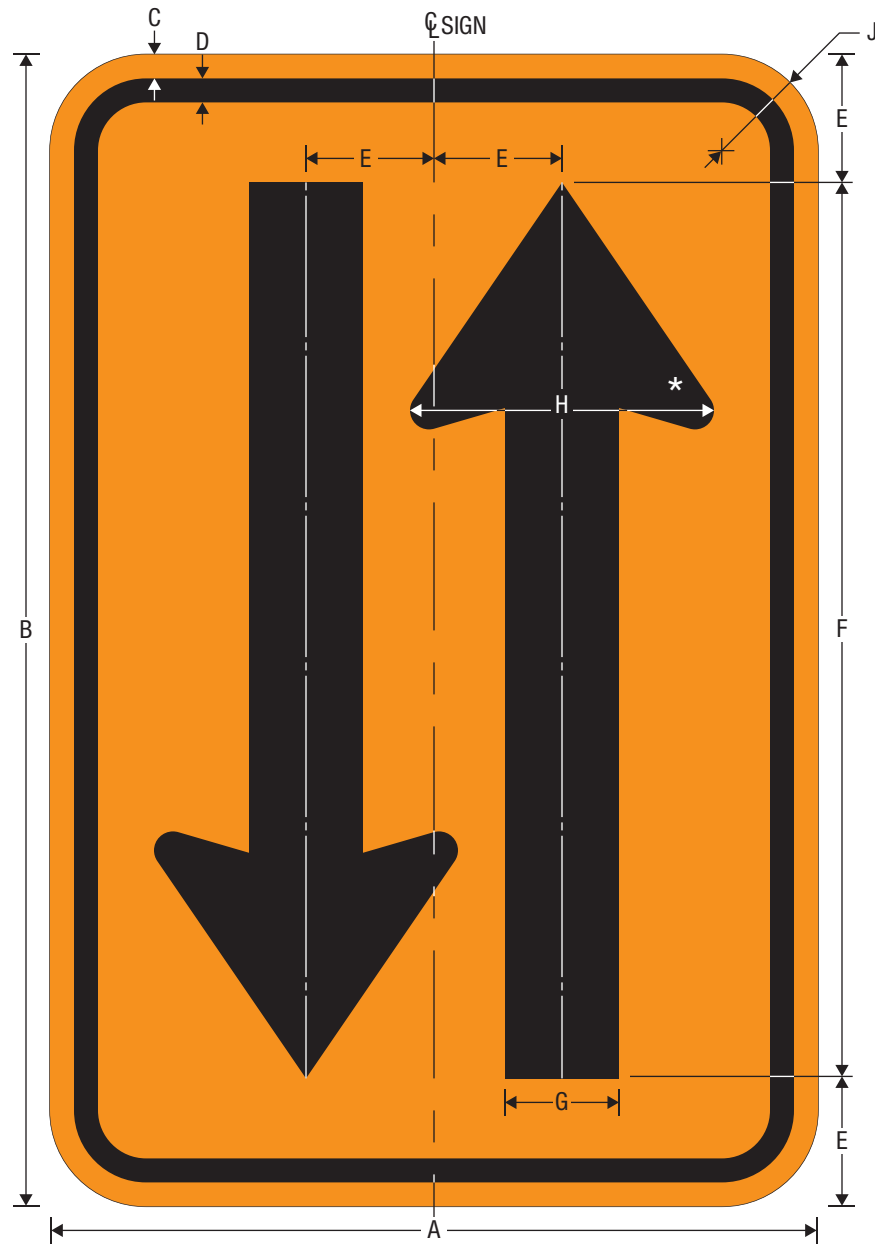
W6-4 NARROW TWO-WAY TRAFFIC
