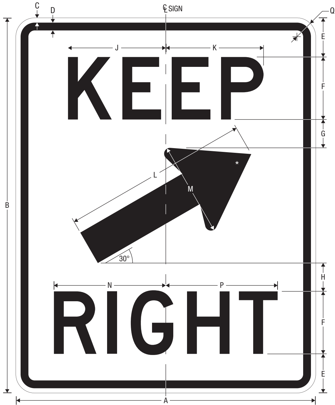
R4-7b KEEP RIGHT
