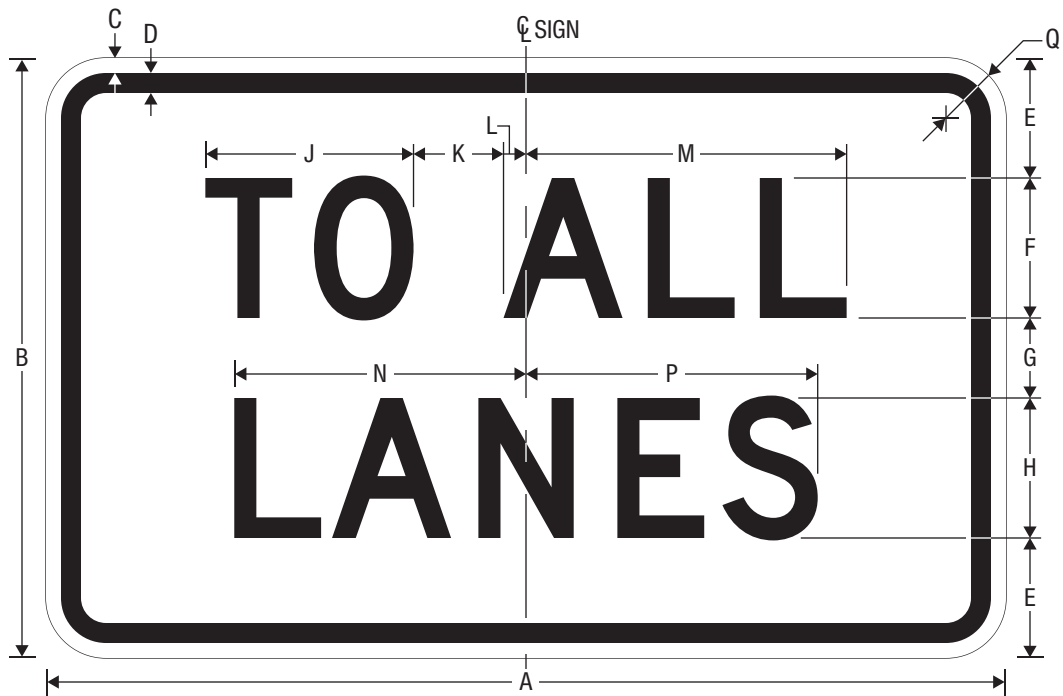
R1-2cP TO ALL LANES (PLAQUE)
