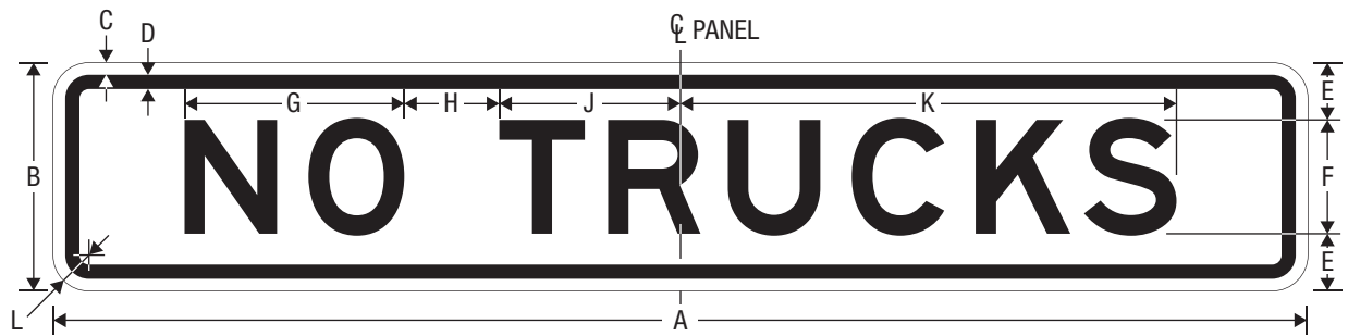
R3-51aP NO TRUCKS (PLAQUE)
