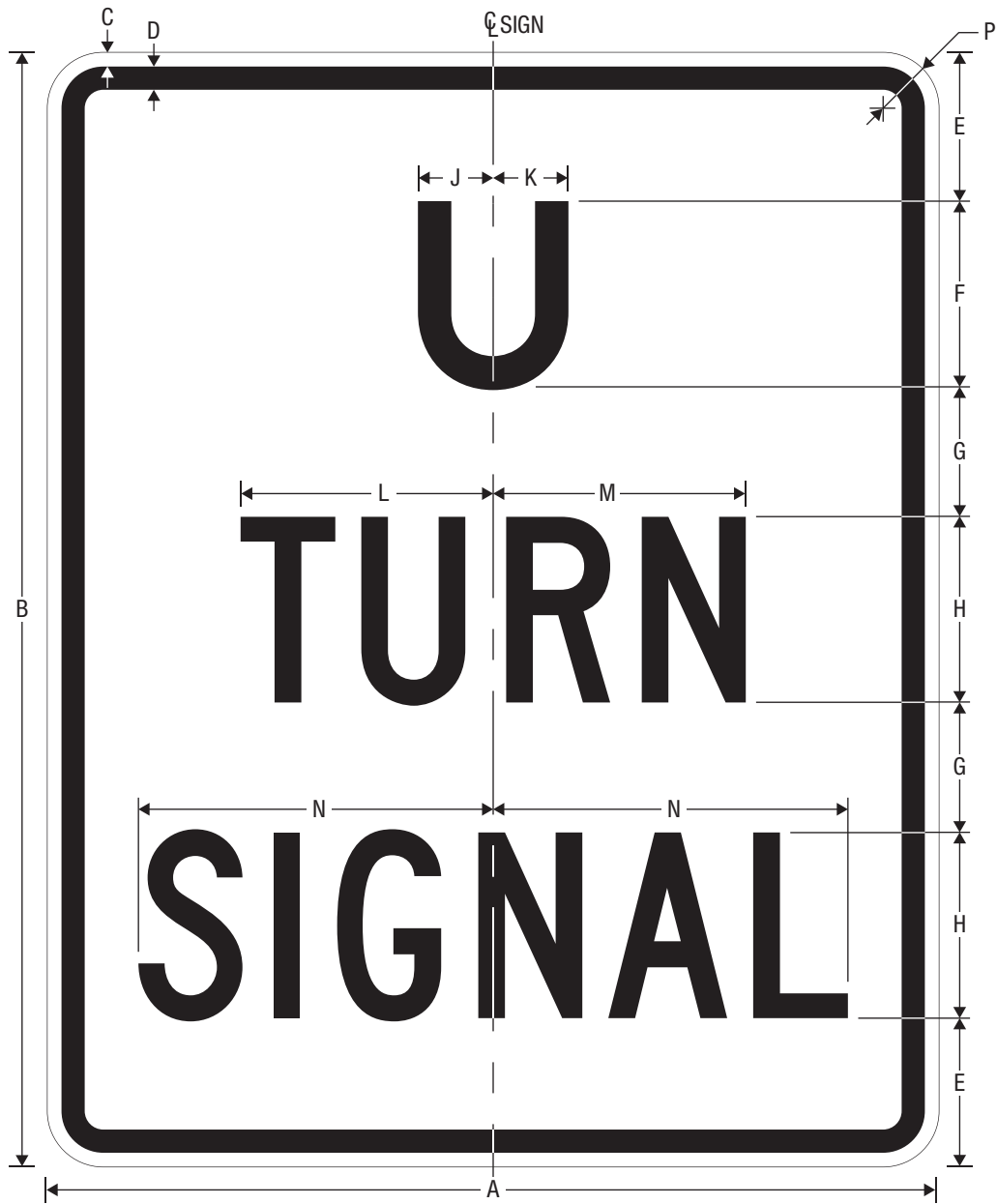
R10-10a U TURN SIGNAL
