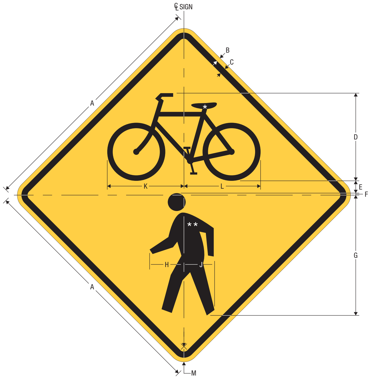
W11-15 TRAIL CROSSING
