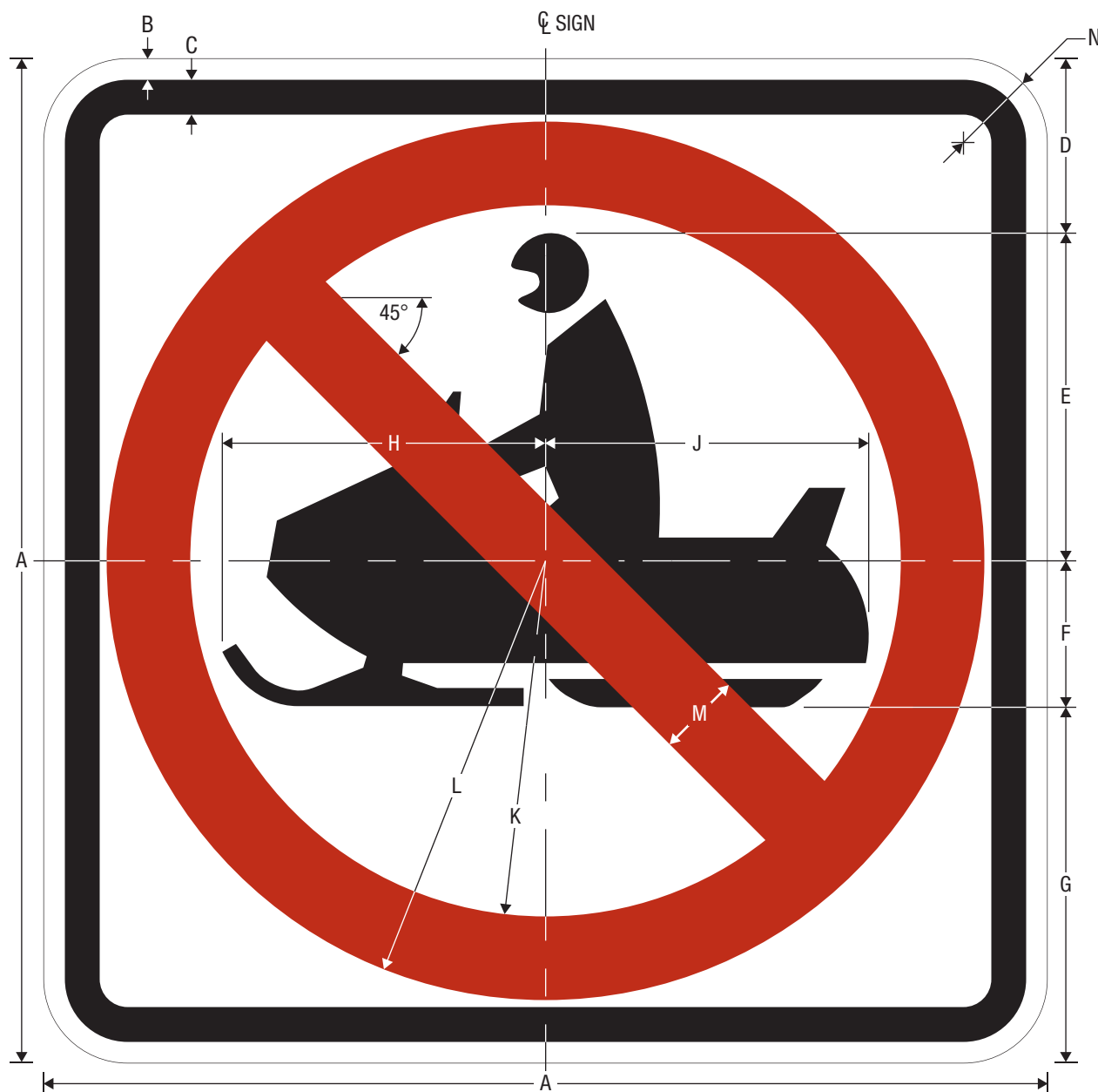
R9-15 NO SNOWMOBILES
