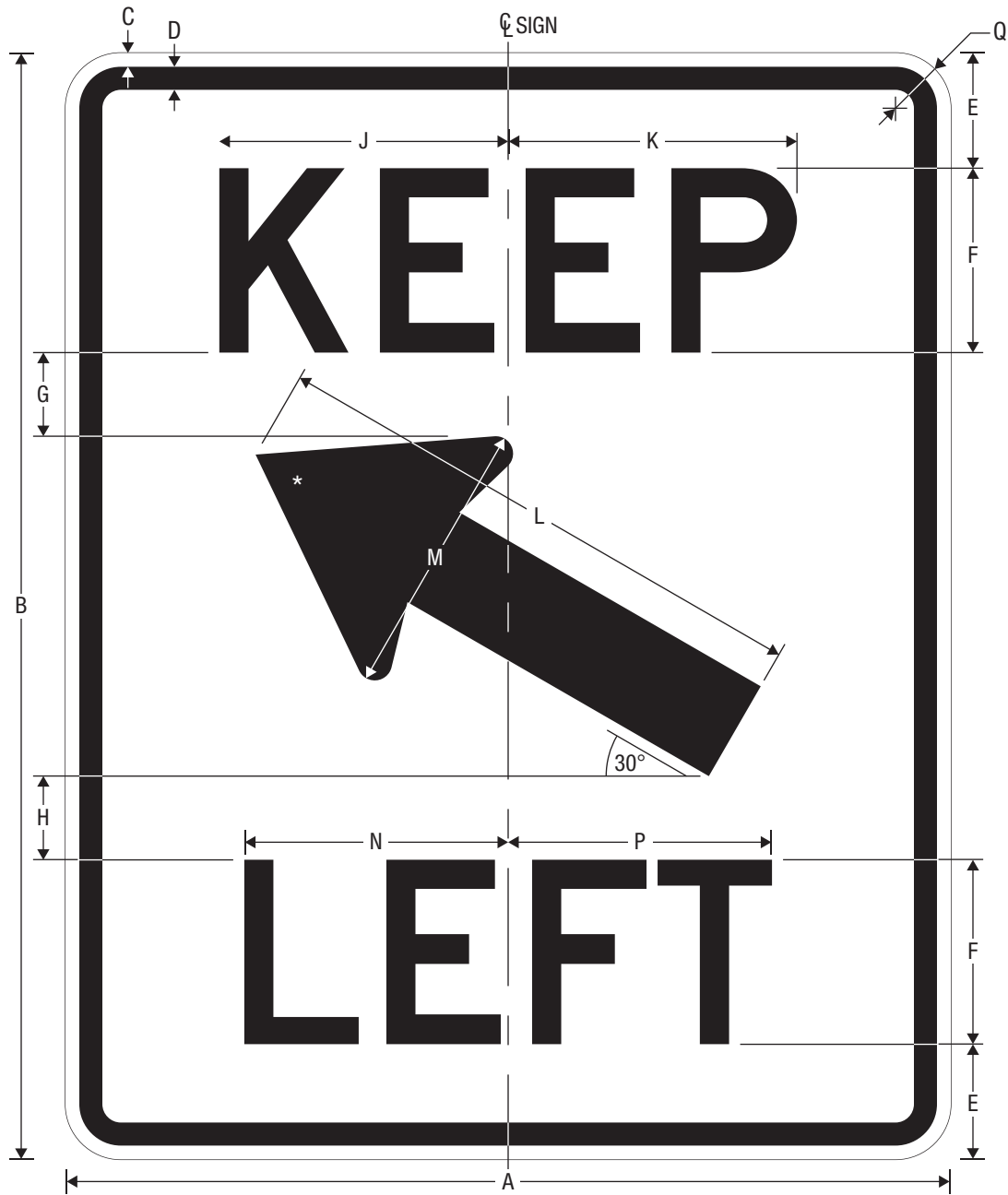
R4-8b KEEP LEFT
