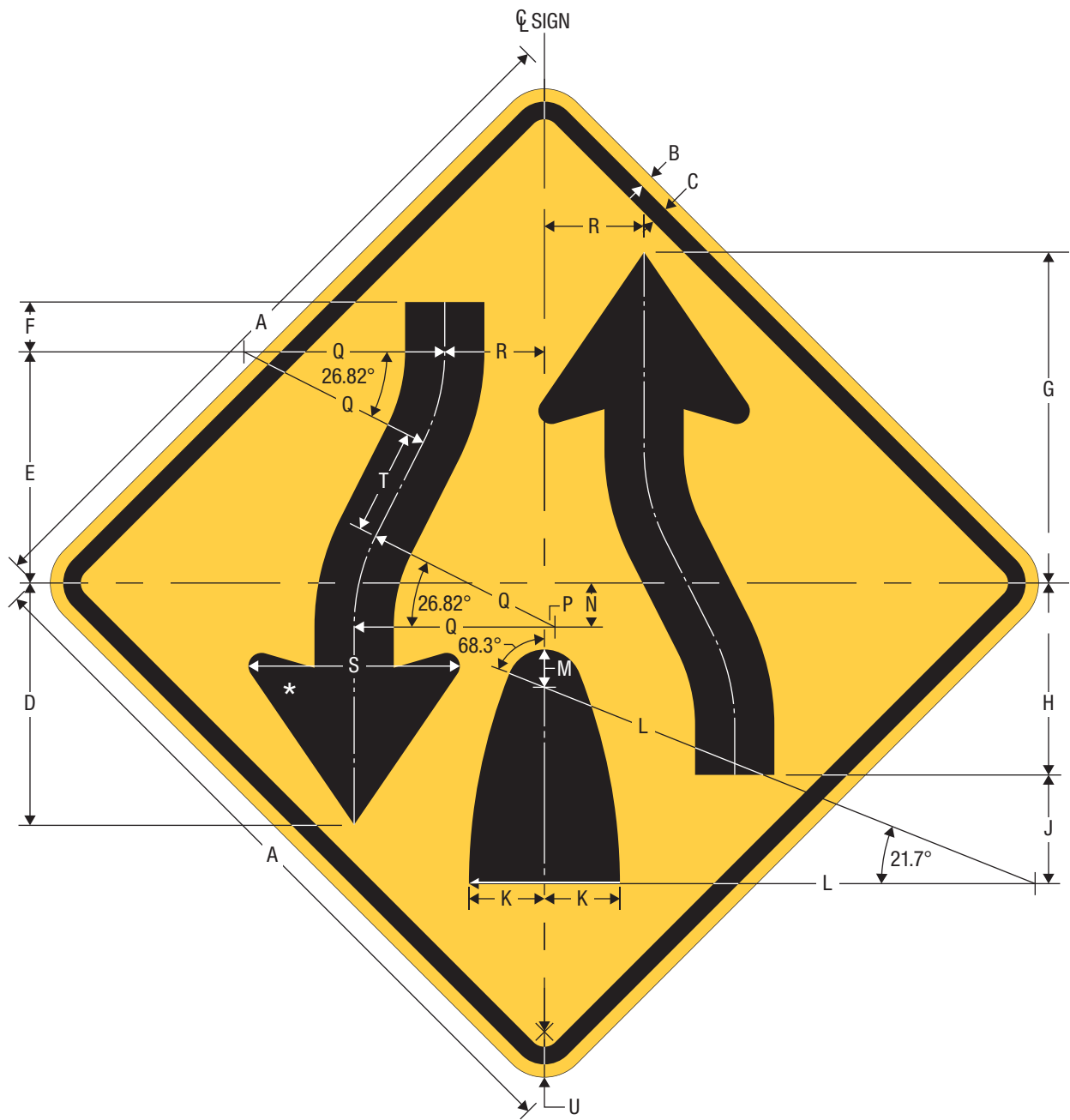
W6-2 DIVIDED HIGHWAY ENDS
