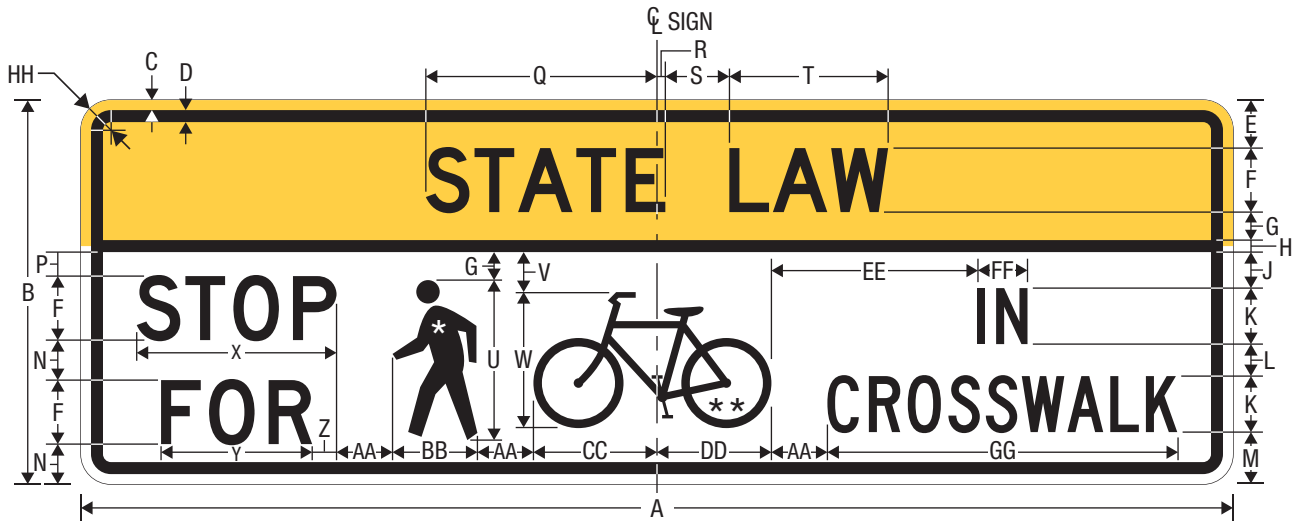
R1-9e OVERHEAD TRAIL CROSSING - STOP
