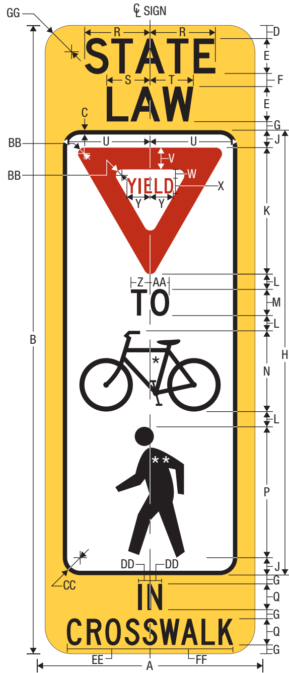
R1-6d IN-STREET TRAIL CROSSING - YIELD
