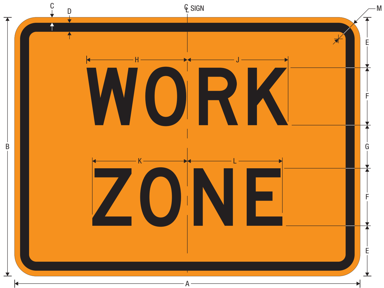
G20-5aP WORK ZONE (PLAQUE)
