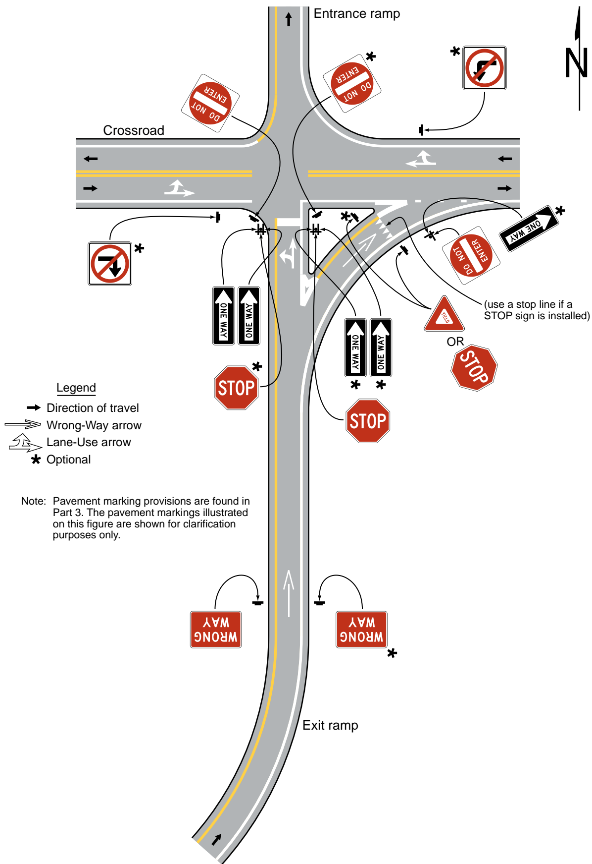
Figure 2B-15. Example of Application of Regulatory Signing and Pavement Markings at an Exit Ramp Termination to Deter Wrong-Way Entry
