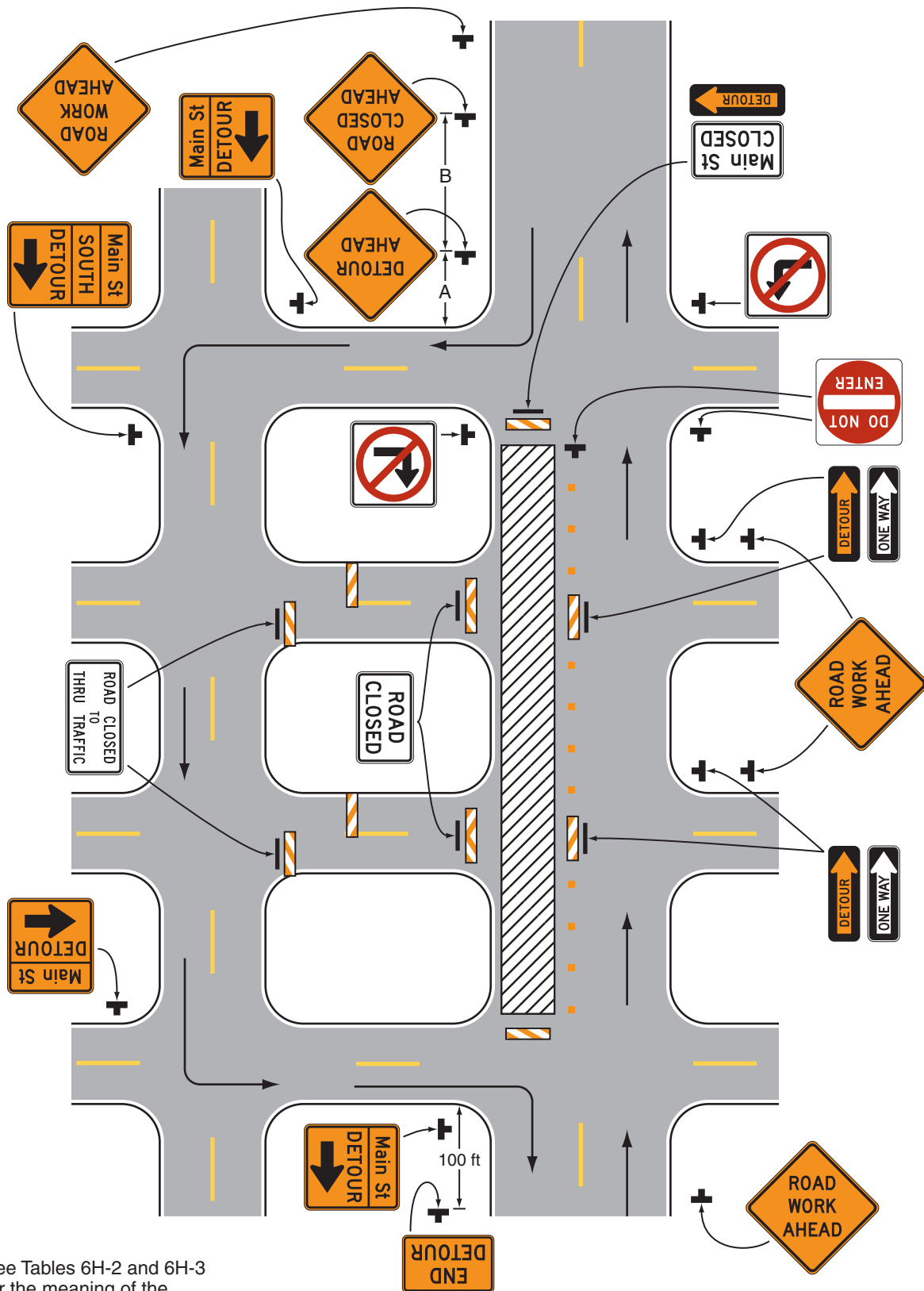
Typical Application 19
