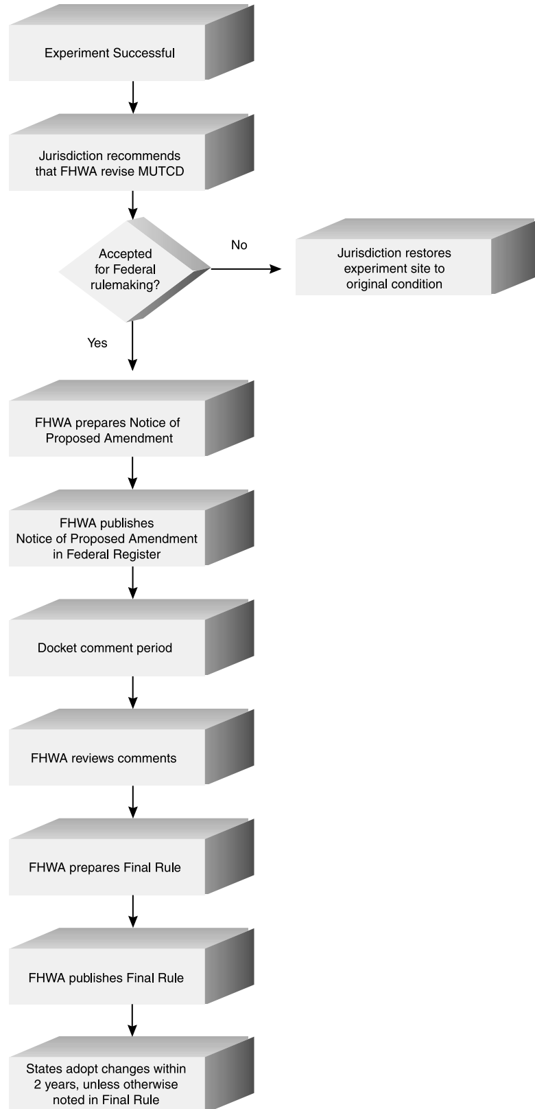
Figure 1A-2. Typical Process for Incorporating New Traffic Control Devices into the MUTCD
