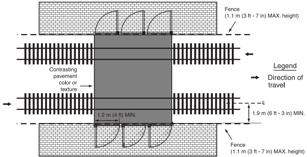
Figure 10D-6. Example of Swing Gates
