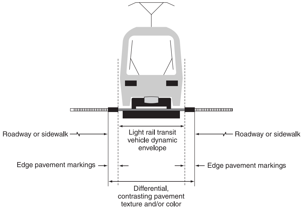
Figure 10C-6. Light Rail Transit Vehicle Dynamic Envelope
