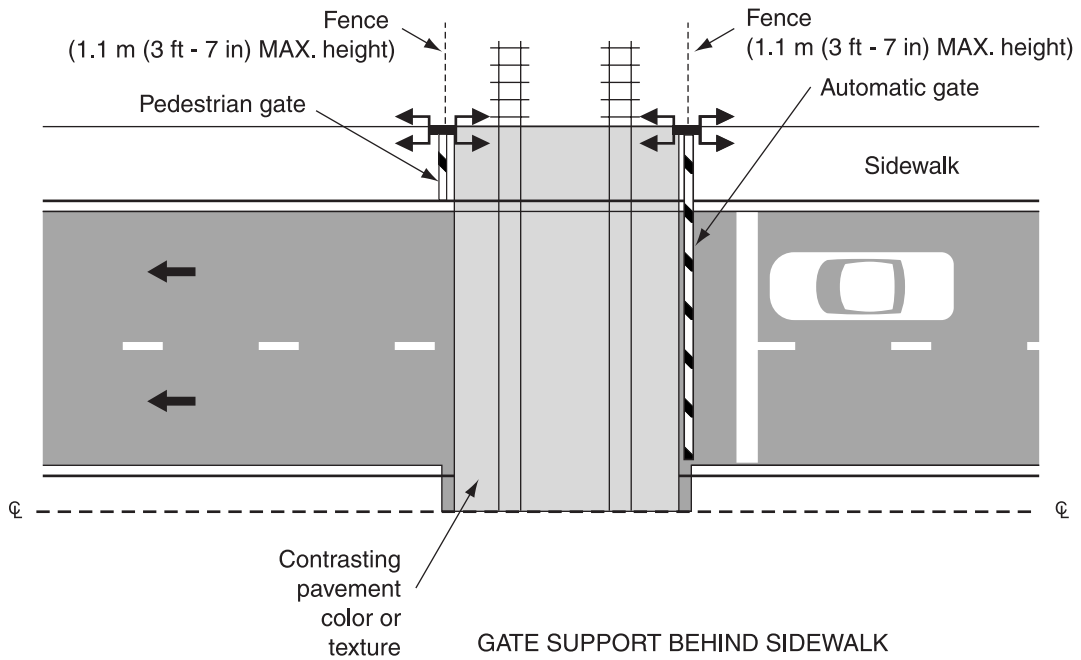
Figure 10D-5. Examples of Placement of Pedestrian Traffic Gates
