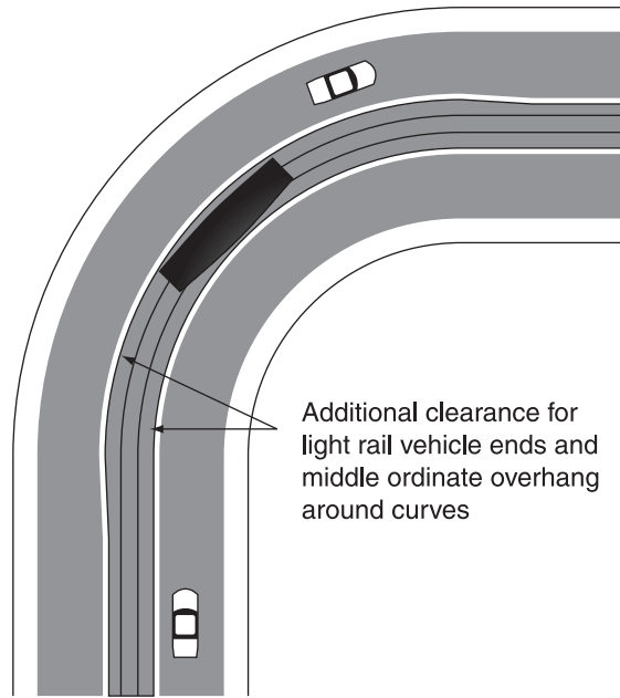
Figure 10C-8. Example of Light Rail Transit Car Dynamic Envelope Pavement Markings
