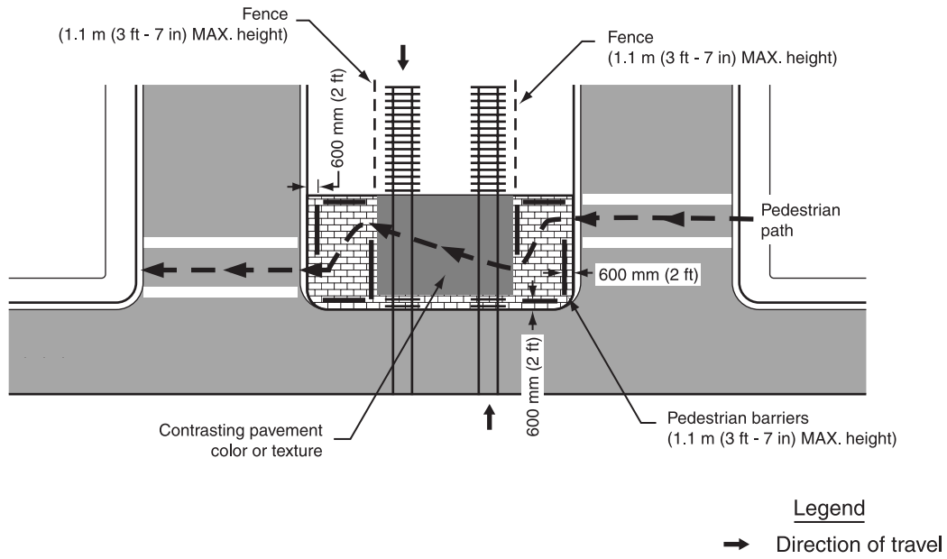
Figure 10D-7. Example of Pedestrian Barriers at an Offset Highway-Light Rail Transit Crossing
