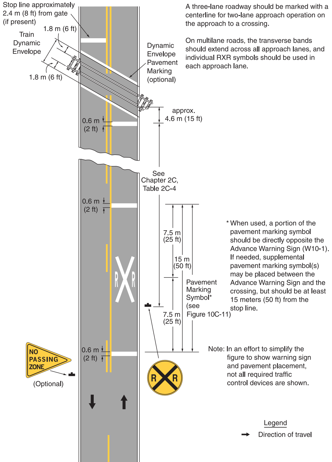
Figure 10C-10. Example of Placement of Warning Signs and Pavement Markings at Highway-Light Rail Transit Grade Crossings
