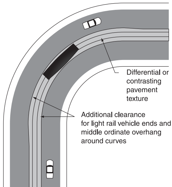
Figure 10C-9. Example of Light Rail Transit Vehicle Dynamic Envelope Contrasting Pavement Texture
