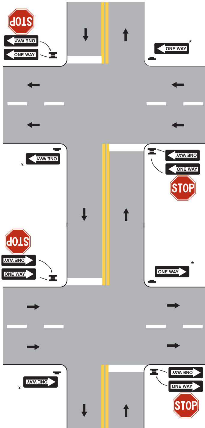
Figure 2B-10. Examples of Locations of ONE WAY Signs
