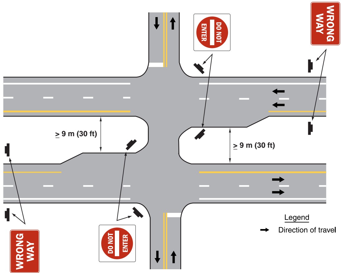
Figure 2B-8. Example of Wrong-Way Signing for a Divided Highway with a Median Width of 9 m (30 ft) or Greater
