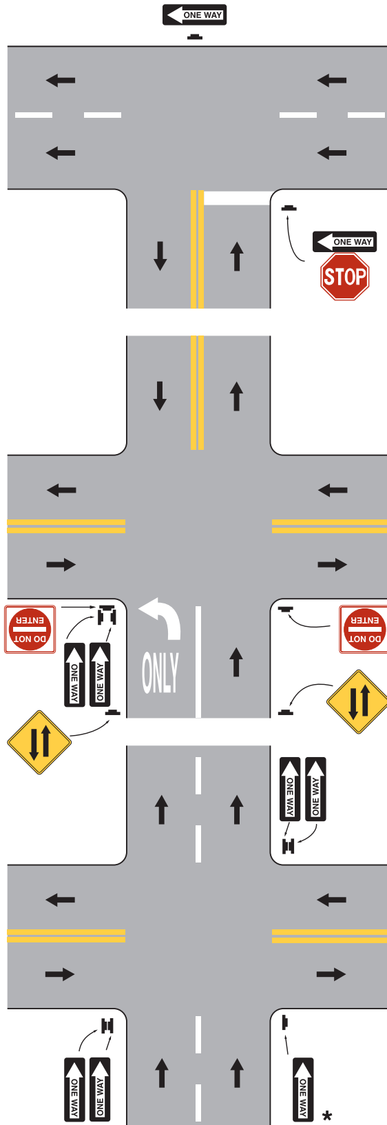
Figure 2B-11. Examples of Locations of ONE WAY Signs
