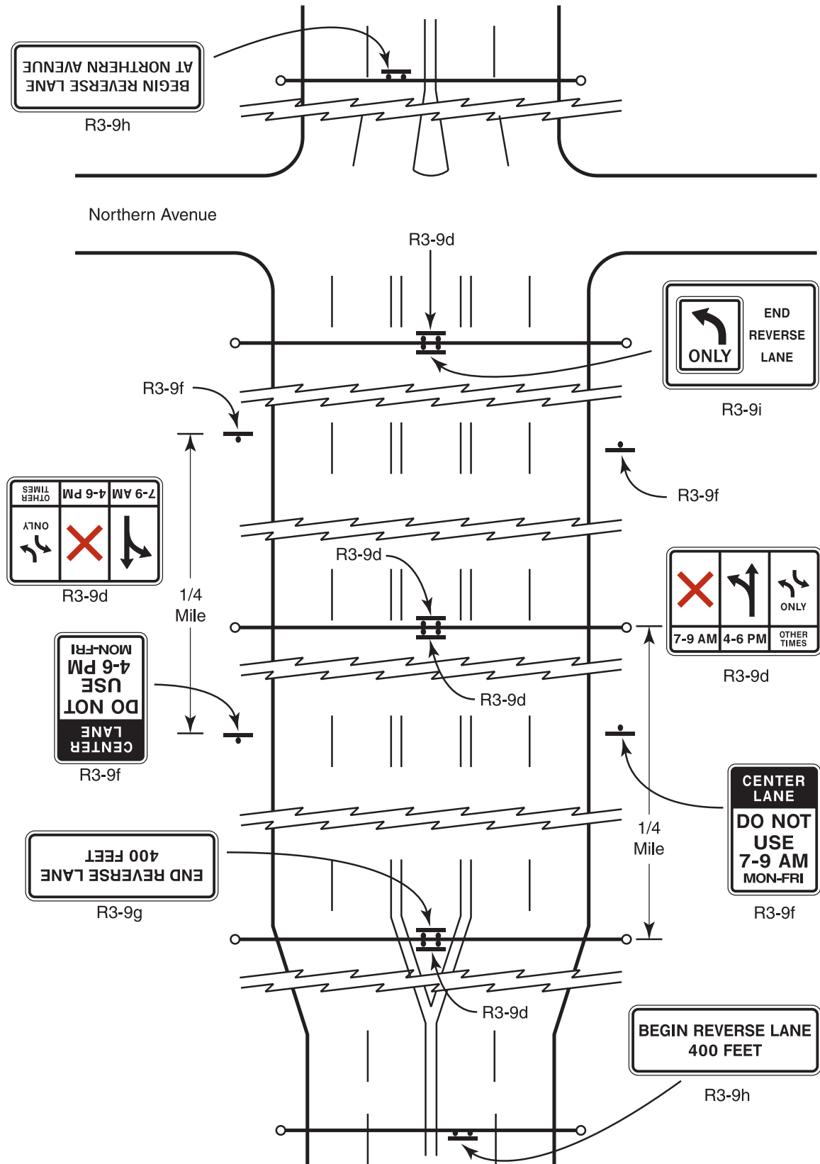
Figure 2B-5. Location of Reversible Two-Way Left-Turn Signs
