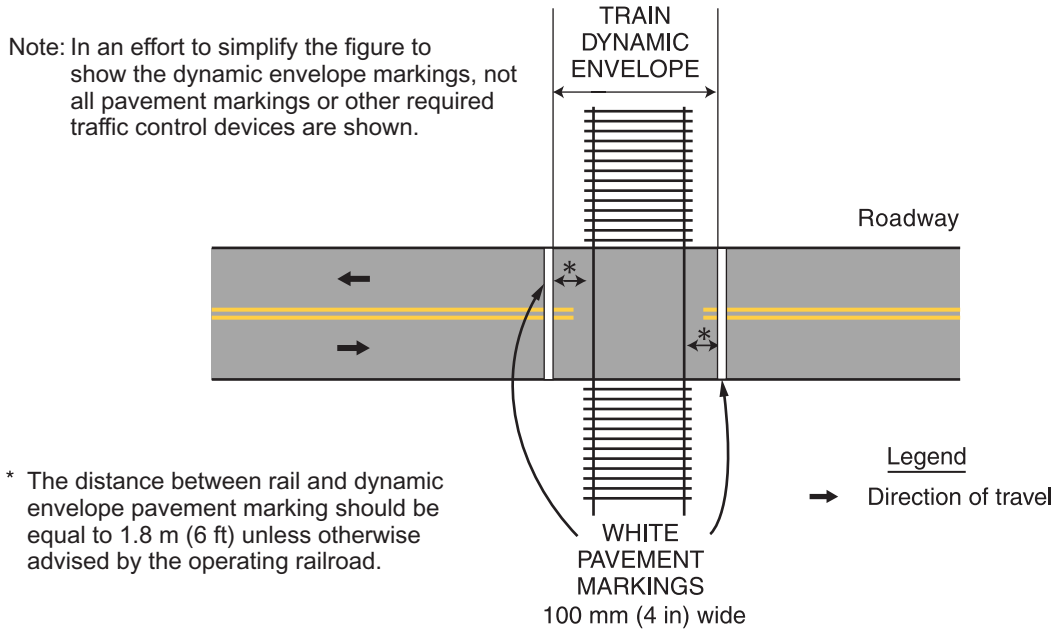
Figure 8B-9. Example of Train Dynamic Envelope Pavement Markings
