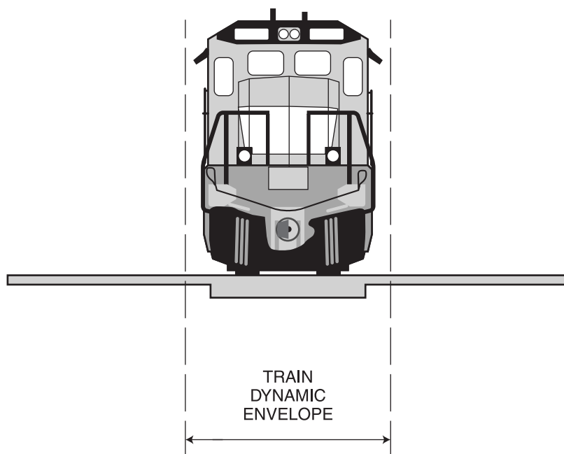
Figure 8A-1. Train Dynamic Envelope
