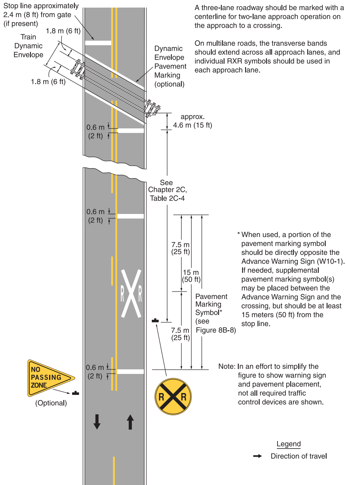
Figure 8B-7. Example of Placement of Warning Signs and Pavement Markings at Highway-Rail Grade Crossings
