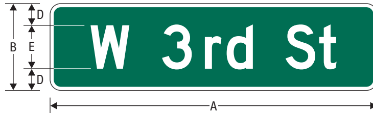
D3-1 (Sheet 1 of 3) Street Name Sign
